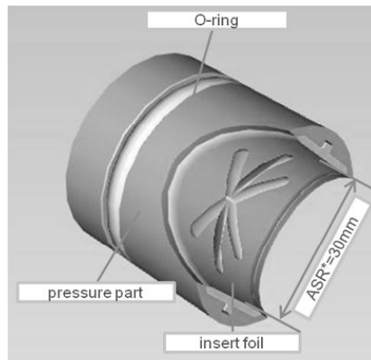
Figure 2: Pressure Piece
