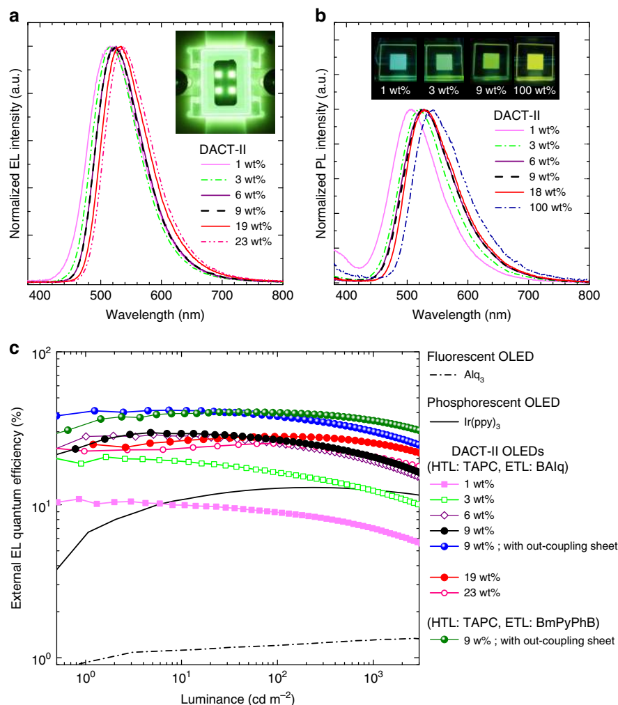
Figure 2 | EL and PL of DACT-II. (a) EL spectra for the DACT-II-x devices . A photograph of EL emission for the DACT-II-9 device is also shown. (b) PL spectra of DACT-II in CBP films and a neat DACT-II film. Photographs of PL emission are also shown. (c) EQE versus luminance for the DACT-II-x devices . EQE values of the Alq 3 device and Ir(ppy) 3 device are also shown.
