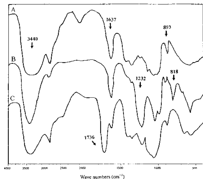
Fig. 2. Comparison of IR Spectra of (A) the Parent Glucan PSGL-I-1A, (B) Sulfated PSGL-I-1A (DS=1.1), and (C) Carboxymethylated PSGL-I-1A (DS=1.11)
