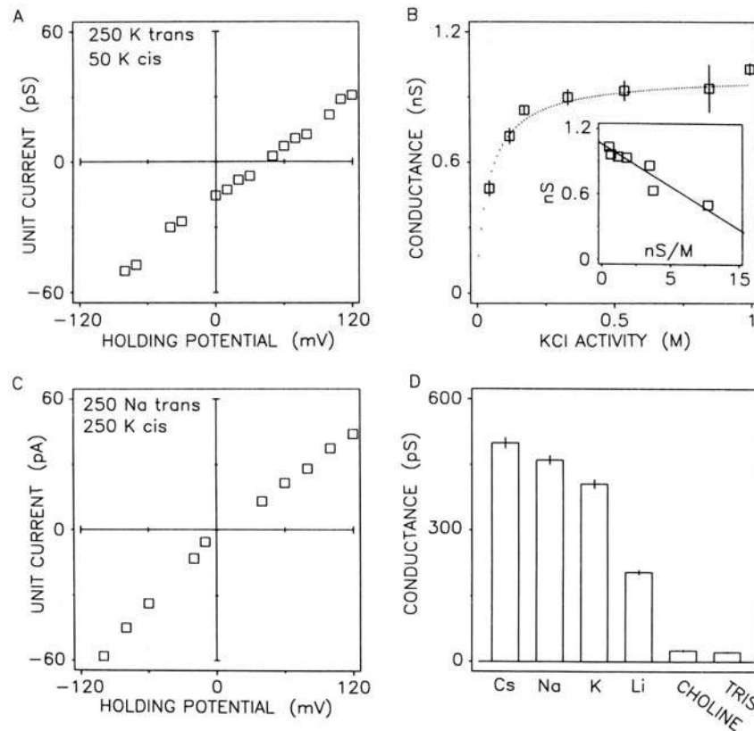
FIGURE 11. Monovalent cation current through ryanodine receptor channels. (A) Single-channel current-voltage relationship for channels recorded in 50 mM CM KCl and 250 mM trans KCl; 10 mM K-HEPES, pH 7.4, was present in both chambers. Current reversal was at +40 \pm 2 mV. The Nernst reversal for K is +39 mV. (B) Saturation of K conductance according to a rectangular hyperbola with K_s = 47.3 mM and \gamma_{\max} = 1.032 nS. The inset is an Eadie-Hofstee plot of K conductance vs. concentration. The line drawn through data points has a slope of -0.0473 M and a y -intercept at 1.032 nS. The concentration of KCl was increased symmetrically in both solutions. (C) Single-channel current-voltage curve for channels recorded in 250 mM cis KCl and 250 mM trans NaCl; 10 mM K-HEPES or Na-HEPES, pH 7.4, was present in the cis and trans sides, respectively. Current reversal was at 0 mV. (D) Single-channel conductance for selected monovalent cations recorded in 50 mM cis and 250 mM trans test cation concentration. Unit conductances were 500 \pm 12 , 461 \pm 10 , 406 \pm 10 , 205 \pm 5 , 26 \pm 2 , and 22 \pm 1 pS for Cs, Na, K, Li, choline, and Tris, respectively. Cl salts were used in all experiments.
