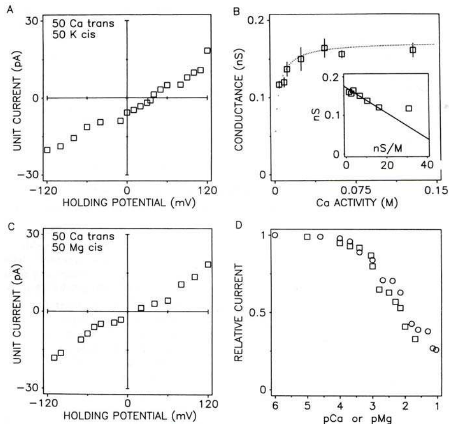
FIGURE 12. Divalent cation current through ryanodine receptor channels. (A) Single-channel current-voltage curve for channels recorded in 50 KCl, 10 mM K-HEPES, pH 7.4 CM, and 50 CaCl 2 , 10 mM Ca-HEPES, pH 7.4 trans . The slope conductance is 123 \pm 3 pS. The current reversal is +39 mV, which gives a permeability ratio P_{Ca}/P_K = 6.6 . (B) Saturation of Ca conductance according to a rectangular hyperbola with fitted parameters K_d = 3 mM and \gamma_{max} = 172 pS. The inset is an Eadie-Hofstee plot of Ca conductance vs. concentration. The line drawn through data points has a slope of -0.003 M and a y -intercept at 0.172 nS. The concentration of CaCl 2 was increased symmetrically in both solutions. (C) Single-channel current-voltage curve for channels recorded in 50 mM MgCl 2 , 10 mM Mg-HEPES, pH 7.4 cis , and 50 mM CaCl 2 , 10 mM Ca-HEPES, pH 7.4 trans . Current reversal was at 0 mV. (D) Blockade of K current by Ca and Mg. Channels were recorded at +60 mV in symmetrical 245 KCl, 10 mM K-HEPES, pH 7.4. CaCl 2 (squares) or MgCl 2 (circles) was added to the cis chamber. The IC 50 for both Ca and Mg is 2.5 mM.
