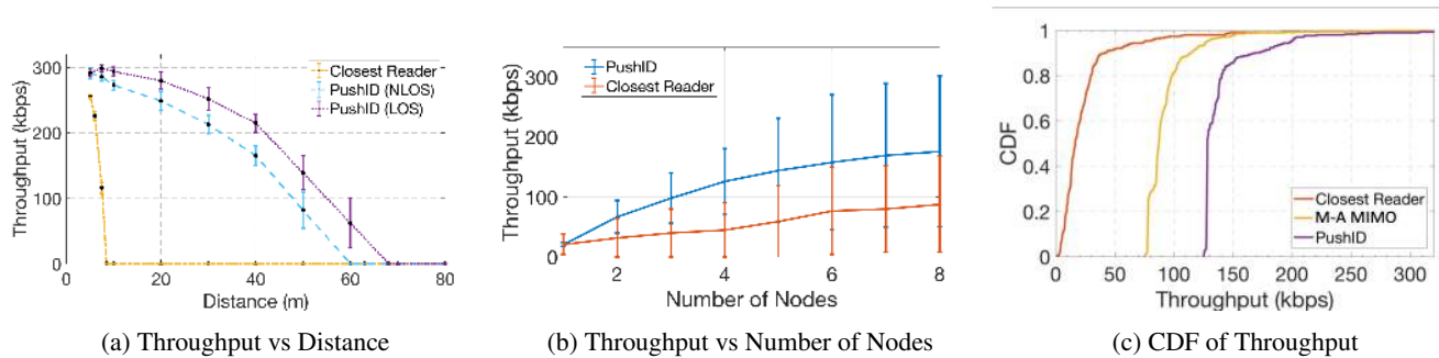
Figure 10: Throughput vs. (a) Distance of closest reader; (b) number of readers; (c) CDF with changing tag orientation.
