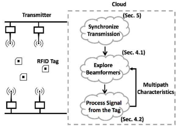
Figure 2: Architecture of PushID
