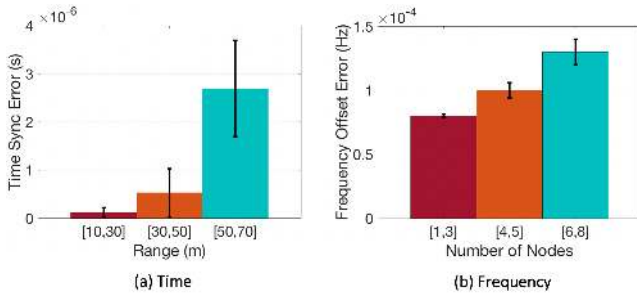
Figure 9: Time and Frequency Synchronization Accuracy
