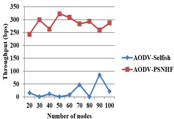
Figure. 5 Throughput under selfish nodes
