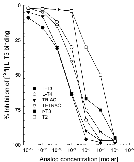
Fig. 2. Representative curves of [ 125 I] L-T3 binding to the purified liver nuclear fraction and its displacement by different thyroid hormone analogs: L-T4, triiodothyroacetic acid (TRIAC), tetraiodothyroacetic acid (TETRAC), 3,3',5'-triiodothyronine (r-T3) and diiodothyronine (T2). Purified toad liver nuclei were incubated with 10 pM [ 125 I] L-T3 under standard assay conditions alone (total binding) or in the presence of increasing concentrations of unlabeled thyroid hormone analogs. Data were plotted as the percentage of relative inhibition of saturable [ 125 I] L-T3 binding to nuclei in the presence of increasing concentrations of unlabeled analogs. Non-specific binding was determined in the presence of 15.4 μM of unlabeled L-T3.
