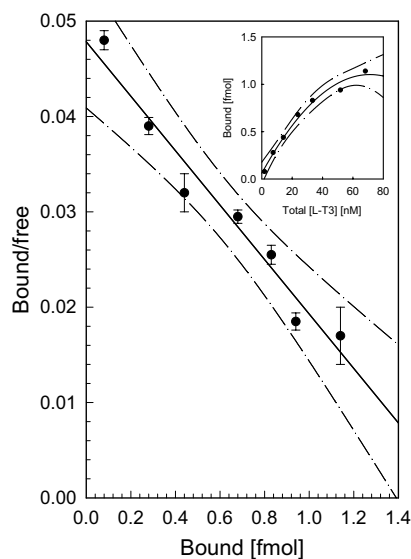
Fig. 1. Scatchard plot of [ ^{125} I] L-triiodothyronine (L-T3) binding in the mature toad liver purified nuclear fraction. The solid line indicates a single class of high affinity binding sites ( \bullet ) having a dissociation constant ( K_d ) of (3.7 \pm 0.9) \times 10^{-10} M and maximum binding capacity ( B_{max} ) of 0.074 \pm 0.013 pmol/mg DNA. K_d and B_{max} were determined by first-order linear regression analysis (solid line) using Sigma Plot software. Data represent mean \pm SEM of four sets of experiments performed in triplicate. The vertical bars denote SEM. Dash-dot line represents 99% confidence interval. Correlation coefficient ( r^2 ) value for the Scatchard plot was 0.96. The inset shows the saturation of the binding sites (solid line) and 99% confidence intervals (dash-dot line) with increasing concentrations of L-T3. Correlation coefficient ( r^2 ) value for the saturation curve was 0.99.
