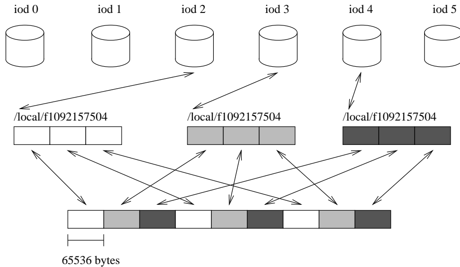
Figure 1: File-striping example
