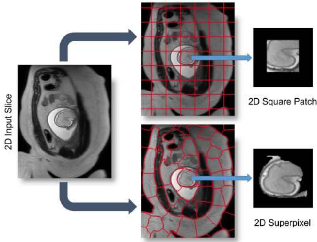
Fig. 5. An illustrative figure showing both square patches and superpixels methods for the patch extraction step. A 2D superpixel shows more flexibility than a square patch in extracting rigid regions or similar voxels. In practice, superpixels are dilated with few pixels to include some contextual information in order to increase the accuracy of the patch to volume registration step.
