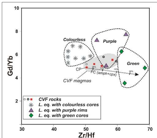
FIGURE 13 | Gd/Yb vs Zr/Hf ratios of melts equilibrated with clinopyroxenes. The compositional field of Calatrava Volcanic Field (CVF) magmas is also shown for comparison. The clinopyroxene compositions used for calculations are averaged values for selected colorless megacrysts (115603, 114404, 111639) and phenocryst cores (115605, 116596), together with green phenocryst cores (116596) and pyroxenites (115601, 115591). Purple rims overgrow phenocrysts (115605, 116596) and pyroxenite crystals (115591) (see Supplementary Table S2 for averaged clinopyroxene values). The C_0 for the fractional crystallization model is the CAL-73 nephelinite (from the Cerro Pelado volcano, CP in figure). The arrow represents the trend of chemical evolution of melts based on the fractionation model (up to 80% of fractional crystallization) considering extraction of 45% clinopyroxene + 45% amphibole + 10% olivine.
