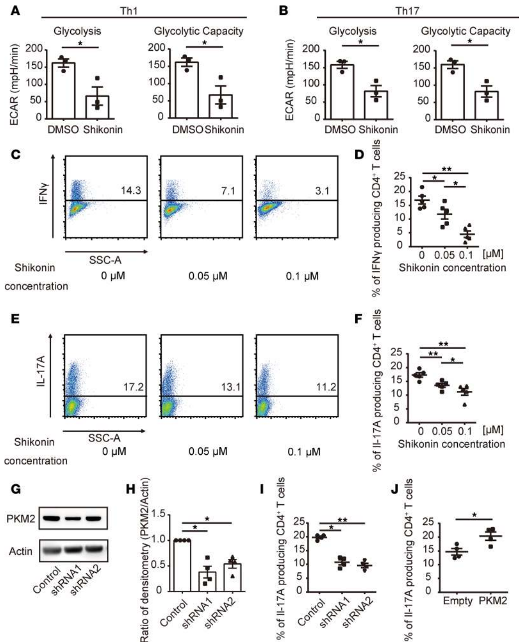
Figure 3. PKM2 promotes in vitro Th1 and Th17 differentiation. (A–F) Naive CD4 ^+ T cells were cultured for 3 days under Th1- and Th17-polarizing conditions and various concentration of shikonin were added on day 0. (A and B) Extracellular acidification rate (ECAR) in Th1 (A) and Th17 cells (B) with or without shikonin was measured on day 3. Cumulative data are shown (mean \pm SEM); n = 3 . (C and E) Representative flow plots of IFN- \gamma -producing (C) and IL-17A-producing (E) CD4 ^+ T cells are shown. (D and F) Cumulative data of IFN- \gamma -producing (D) and IL-17A-producing (F) CD4 ^+ T cells are shown (mean \pm SEM); n = 5 . (G–I) Naive CD4 ^+ T cells were cultured for 4 days under Th17-polarizing conditions and transfected with control shRNA or Pkm2 -specific shRNA on day 1. (G) PKM2 and actin protein expression on day 3 was assessed by Western blotting. Representative blots are shown. Data are representative of 4 experiments. (H) Cumulative data of the Western blotting densitometric ratio (PKM2/actin) are shown (mean \pm SEM); n = 4 . (I) Cumulative data of flow plots of IL-17A-producing CD4 ^+ T cells are shown (mean \pm SEM); n = 4 . (J) Naive CD4 ^+ T cells were cultured for 3 days under Th17-polarizing conditions and transfected with empty vector or mouse PKM2-expressing vector on day 1. Cumulative data of IL-17A-producing CD4 ^+ T cells are shown (mean \pm SEM); n = 4 . * P < 0.05 ; ** P < 0.01 by 2-tailed t test (A, B, and J) or 1-way ANOVA with Bonferroni’s multiple-comparisons test (D, F, H, and I).
