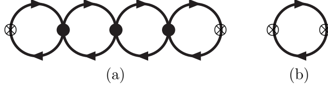
Figure 1: The type of diagrams in large N_c that contribute to the two-point function. \otimes indicates and insertion of an external current and \bullet indicates the ENJL four-quark vertex. (a) the full two-point function. (b) The one-loop two-point function.
