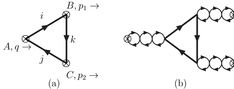
Figure 2: The \Pi^+ contribution to a generic three-point function. (a) The flavour and momentum flow indicated on a one-loop diagram. (b) A generic large N_c diagram with the resummation in terms of bubbles. Note that the resummation leads to full two-point functions.
