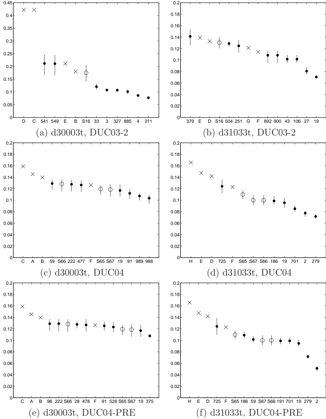
Figure 8. ROUGE-SU4 recall scores plotted with 95% confidence intervals (lines) for the human ( \times ), summarization module ( \circ ) and QCS ( \bullet ) summaries for clusters d30003t and d31033t. The scores appear in descending order of average score from left to right.
