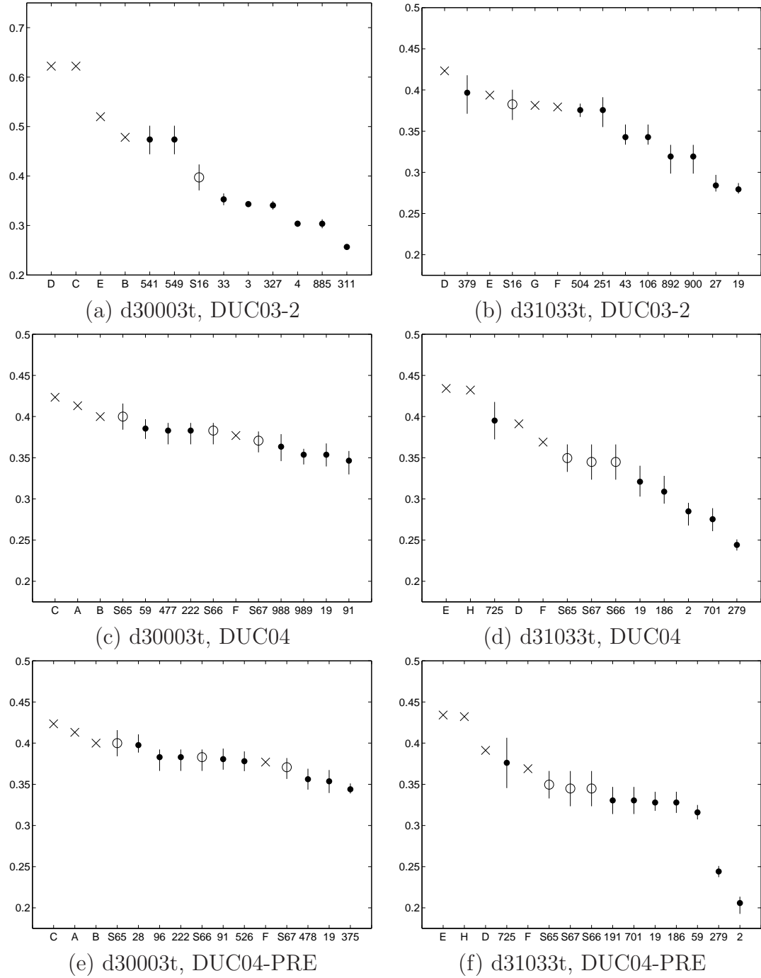
Figure 6. ROUGE-1 recall scores plotted with 95% confidence intervals (lines) for the human (x), summarization module (o) and QCS (•) summaries for clusters d30003t and d31033t. The scores appear in descending order of average score from left to right.
