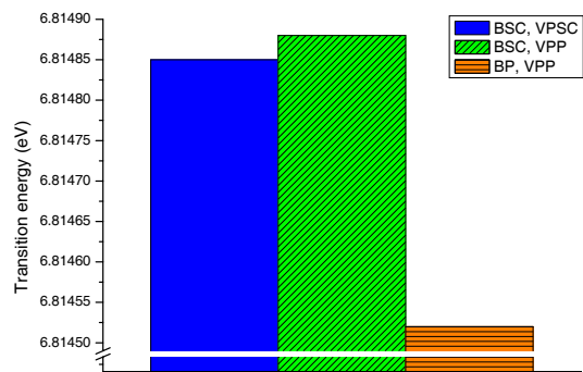
Fig. 10. Changes in the 7p^5 8s \ ^3P_1 \rightarrow 7s^2 7p^6 \ ^1S_0 transition energy with respect to the approximation made, for element 118. BSC: Breit self-consistent. VPSC: Uehling potential self consistent. BP: Breit in perturbation. VPP: Uehling vacuum polarization in perturbation.
