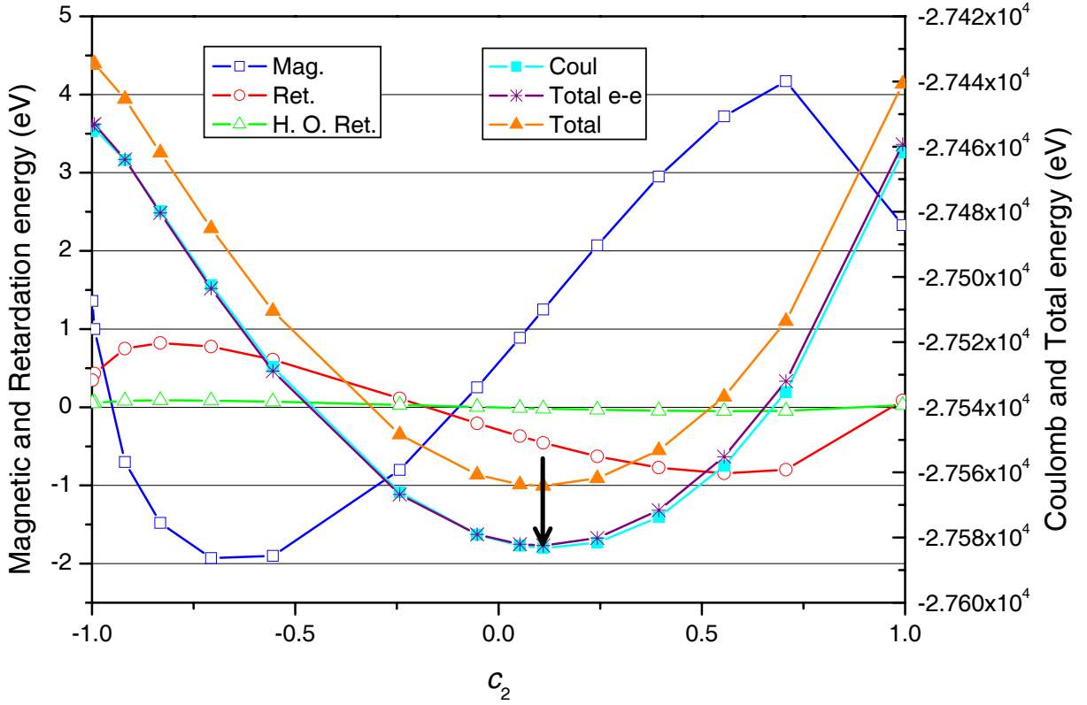
Fig. 4. Variation of the different contributions to the energy as a function of the mixing coefficient c_2 , for the 1s2p\ ^3P_1 level at Z = 40 . The arrow indicates the position of the 1s2p\ ^3P_1 energy, at the minimum around c_2 = 0.104 . Left axis: “Mag.”: Magnetic energy, Eq. (3b). “Ret.”: Breit retardation, Eq. (4). “H. O. Ret.”: higher-order retardation. Right axis: “Coul.”: Coulomb energy Eq. (3a). “Total e-e”: sum of the 4 preceding contributions. “Total”: total level energy including all QED corrections.
