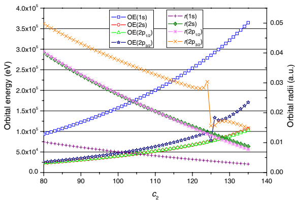
Fig. 8. Orbital radii (right axis) and one-electron energies (left axis) for Be-like ions
