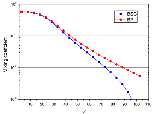
Fig. 3. Variation with Z of mixing c_2 coefficient for the 1s2p^3 P_1 level of helium-like ions. BP: Only the Coulomb interaction is used in the SCF process. BSC: The full Breit interaction is used in the SCF process
