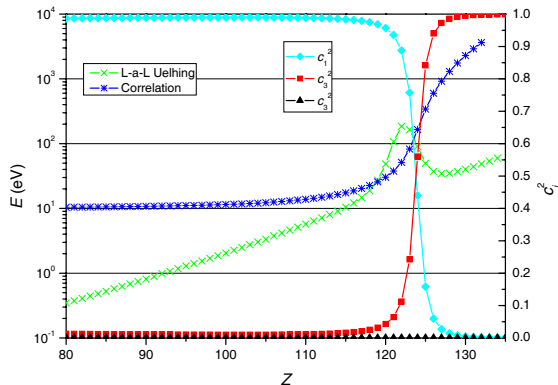
Fig. 7. Loop-after-loop Uehling contribution to berylliumlike ions ground state energy (changed of sign), obtained by including the Uehling potential in the SCF. The intrashell correlation energy is also plotted (left axis), as well as the square of the mixing coefficients of the 1s^2 2s^2 J = 0 , 1s^2 2p^2_{1/2} J = 0 and 1s^2 2p^2_{3/2} J = 0 configurations (right axis).
