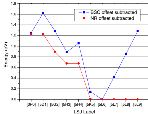
Fig. 1. Non-relativistic offset on the ground configuration of uranium. “Ener. (BSC off. sub)”: total MCDF energy, with all QED corrections, using the full Breit operator in the SCF process, relative to the 5f^36d7s^2 {}^5L_6 energy to which the non-relativistic offset has been subtracted. “Ener. (NR off. sub)”: Total non-relativistic energy, to which the non-relativistic offset for members of the same LS multiplet has been subtracted, relative to the 5f^36d7s^2 {}^5L_6 energy. The two {}^5H_J and the four {}^5L_J levels have thus identical non-relativistic energy as it should be. Uncorrected energy and NR offset are displayed in Table 2
