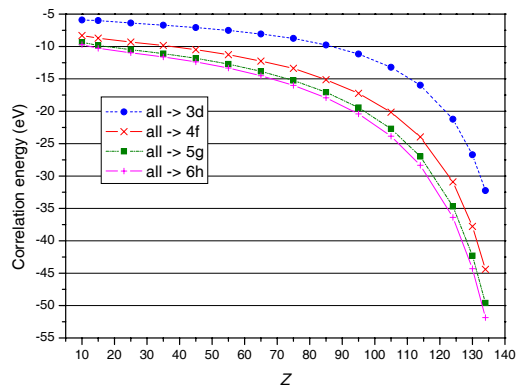
Fig. 9. Total correlation energy for neonlike ions, with the Breit interaction included in the SCF, as a function of the most excited orbital included in the basis set.
