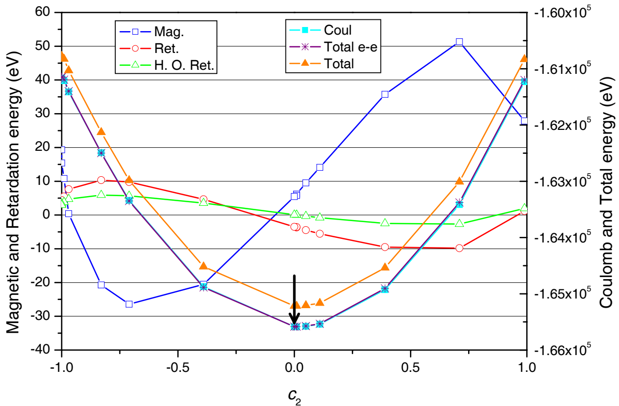
Fig. 5. Variation of the different contributions to the energy as a function of the mixing coefficient c_2 , for the 1s2p\ ^3P_1 level at Z = 92 . The arrow indicates the position of the 1s2p\ ^3P_1 energy, at the minimum around c_2 = 0.002 . Left axis: “Mag.”: Magnetic energy, Eq. (3b). “Ret.”: Breit retardation, Eq. (4). “H.O. Ret.”: higher-order retardation. Right axis: “Coul.”: Coulomb energy Eq. (3a). “Total e-e”: sum of the 4 preceding contributions. “Total”: total level energy including all QED corrections.
