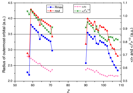
Fig. 13. Variation of \langle r \rangle , \sqrt{\langle r^2 \rangle} (right scale), of the radius of the outermost orbital \langle r_{\text{out}} \rangle and of the maximum of the charge density of the outer orbital (Rmax. dens.) (left scale) as a function of the atomic number Z .
