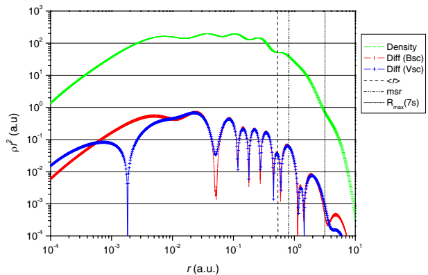
Fig. 11. Total electronic density of \text{Fm}^+ . The vertical lines represents, from left to right the mean radius, the mean spherical radius (“rms”) and the mean radius of the outermost orbital (7s). “Density”: total electronic density Eq. (10). “Diff (Bsc)”: absolute value of the variation in the density due to the inclusion of the Breit interaction in the SCF. “Diff (Vsc)”: absolute value of the variation in the density due to the inclusion of the Uehling potential in the differential equations (NB: the dip in the curve correspond to sign changes of the correction).
