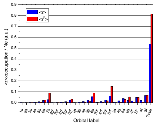
Fig. 12. Contribution to the mean radius \langle r_{\text{at.}}^{(p)} \rangle to \text{Sg}^+ of individual values of \varpi_i \langle r_{n_i, l_i, j_i}^{(p)} \rangle for the different orbitals and p = 1 and 2, together with the total values on the right. Stared orbital labels correspond to the orbital with j = l - \frac{1}{2} .
