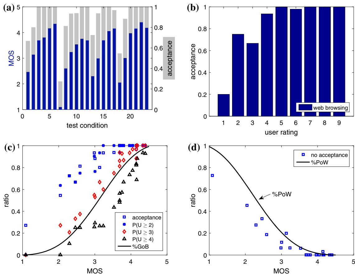
Fig. 5 Task-Related Web QoE and Acceptance. Results of the task-related web QoE and acceptance study (Schatz and Egger 2014) in “ \theta -Acceptability derived from user ratings”. The data is based on a subjective lab experiment in which participants had to browse four different websites at different network speeds resulting in different levels of experienced responsiveness. The network speeds determined the page load times while browsing and executing a certain task. Defined tasks for each technical condition should stimulate the interaction between the web site and the subject for each test condition, see Table 3. In total, there are 23 different test conditions in the data set. The overall quality for each test condition was evaluated by 10–30 subjects on a discrete 9-point scale which was subsequently mapped into a 5-point ACR scale. Furthermore, subjects gave their opinion on the acceptance (yes/no) of that test condition. a MOS & Acceptance per Condition. The blue bars in the foreground depict the MOS values per test condition on the left y-axis. The grey bars in the background depict the acceptance values for that test condition on the right axis. While the acceptance values reach the upper bound of 100 %, the maximum MOS observed is 4.39. The minimum MOS over all test conditions is 1.09, while the minimum acceptance ratio is 27.27 %. b Acceptance per Rating Category. The users are rating the overall quality on a 9-point ACR scale and
