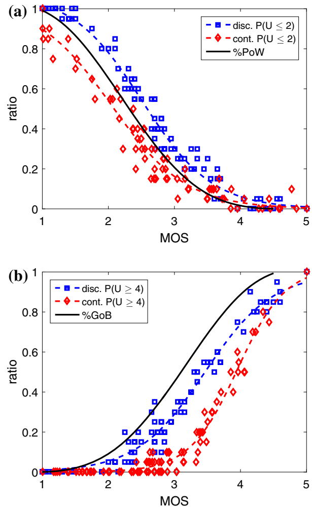
Fig. 8 Speech QoE Results of the speech QoE study Köster et al. (2015). For the 86 test conditions, the MOS and %PoW, %GoB values were computed over the 20 subjects for the discrete 5-point ACR scale (Fig. 6) and the extended continuous scale (Fig. 7). The results for the discrete scale are marked with ‘square’, while the QoE measures for the continuous scale are marked with ‘diamond’. The dashed lines represent logistic fitting functions of the subjective data. a %POW-MOS Plot. The markers depict the MOS and the ratio P(U \leq 2) from the subjective study on the discrete and the continuous scale. The solid black line shows the %PoW ratio depending on MOS for the E-model. The E-model underestimates the measured %PoW on the discrete scale which is larger than the %PoW on the continuous scale. b %GoB-MOS Plot. The markers depict the MOS and the ratio P(U \geq 4) from the subjective study on the discrete and the continuous scale. The solid black line shows the %GoB ratio depending on MOS for the E-model. The E-model overestimates the ratio of satisfied users on the discrete scale which is smaller than the %GoB on the continuous scale
