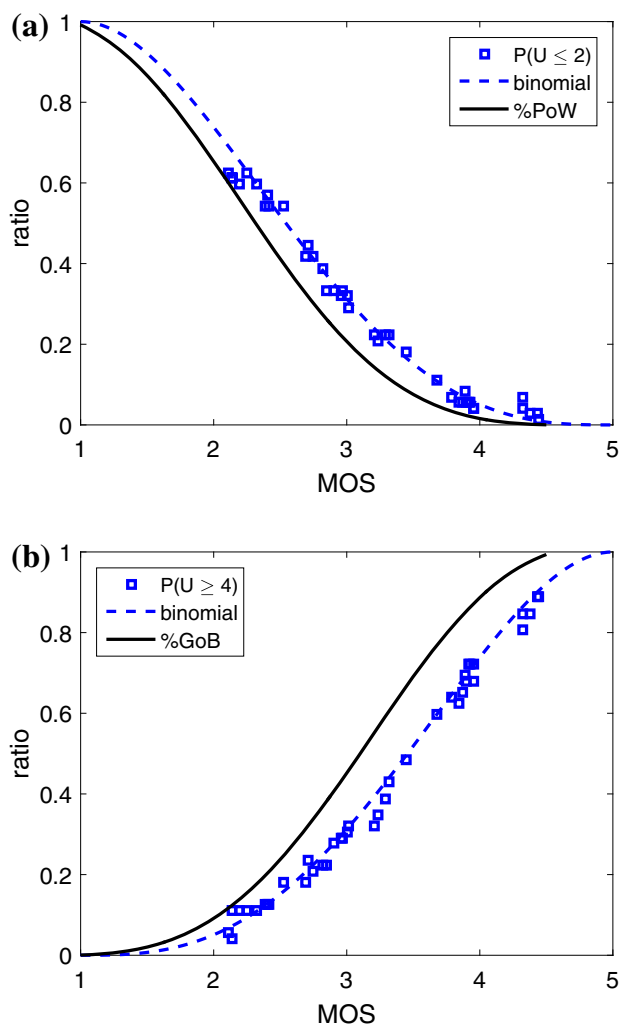
Fig. 13 Web QoE for PLT only. Results of the web QoE study Hößfeld et al. (2011). The page load time was influenced for each test condition and 72 subjects rated the overall quality on a discrete 5-point ACR scale. Each user viewed 40 web pages with different images on the page and PLTs from 0.24 to 1.2 s resulting into 40 test conditions per user. For each test condition, the MOS, SOS, entropy, %GoB, %PoW, as well as 10 and 90 %-quantiles are computed over the opinions of the 72 subjects. a %PoW-MOS Plot. The markers depict the MOS and the ratio P(U \leq 2) for each of the test conditions. The dashed blue line represents the corresponding ratio for the shifted binomial distribution. The solid black line shows the %PoW ratio estimation depending on MOS as defined in Eq. (9). For the minimum MOS 2.111 observed, 37.50 % if the users are rating fair or better. The % PoW estimator underestimates the ratio of dissatisfied users P(U \leq 2) with a maximum difference 11.01 % at MOS 2.731. b %GoB-MOS Plot. The markers depict the MOS and the %GoBi.e. P(U \geq 4) for each test condition of the web QoE study. The dashed blue line represents the corresponding ratio for the shifted binomial distribution. The solid black line shows the %GoB ratio estimation depending on MOS, see Eq. (8). Although the MOS is larger than 4, up to 20 % of the users are rating fair or worse. The %GoB estimator overestimates the ratio of satisfied users P(U \geq 4) with a maximum difference 17.24 % at MOS 3.572
