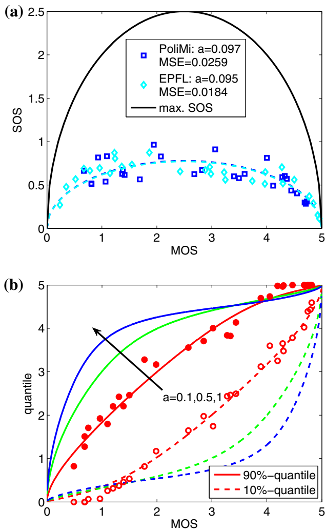
Fig. 10 Video QoE. Results of the video QoE study (De Simone et al. 2009). A continuous rating scales from 0 to 5, cf. Fig. 14, was used in the experiments for subjects evaluating the quality of videos transmitted over a noisy channel (De Simone et al. 2009). The study was repeated in two different labs denoted as ‘EPFL’ and ‘PoliMi’ in the result figures. The packet loss in the video transmission was varied in p_L \in \{0; 0.1; 0.4; 1; 3; 5; 10\} (in %) for four different videos. In total, 40 subjects evaluated 28 test conditions. a SOS-MOS Plot. The markers depict the tuple (MOS, SOS) for each of the 28 test conditions (PoliMi ‘square’ and EPFL ‘diamond’). The dashed lines shows the SOS fitting function with the corresponding SOS parameters for the two labs which are almost identical. When merging the results from both labs, we arrive at the SOS parameter a = 0.10 . But the diversity is lower than for web QoE. Subjects are more sure how to rate an impaired video, while the impact of temporal stimuli, i.e. PLT for web QoE is more difficult to evaluate for subjects. The solid black curve depicts the maximum SOS. b Quantile-MOS Plot. The markers depict the empirically derived 90 %-quantiles ‘filled circle’ and 10 %-quantiles ‘open circle’, respectively. Furthermore, we plot the quantiles depending on MOS for user ratings following a truncated normal distribution and SOS parameter a = 0.1, 0.5, 1 . The SOS hypothesis returns for each MOS value \mu the related SOS value \sigma which allows to compute the quantiles of the truncated normal distribution, i.e. U \sim N(\mu; \sigma; 0; 5) . The solid and dashed lines depict the 90 and 10 %-quantiles, respectively
