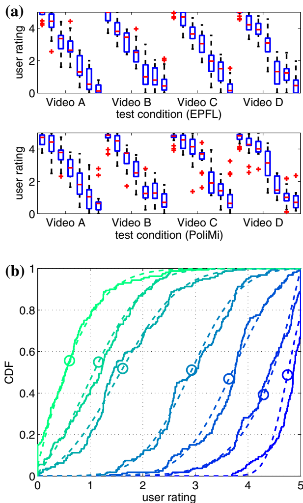
Fig. 15 Video QoE. Results of the video QoE study De Simone et al. (2009). A continuous rating scales from 0 to 5, cf. Fig. 14, was used in the experiments for subjects evaluating the quality of videos transmitted over a noisy channel De Simone et al. (2009). The study was repeated in two different labs denoted as ‘EPFL’ and ‘PoLiMi’ in the result figures. The packet loss in the video transmission was varied in p_L \in \{0; 0.1; 0.4; 1; 3; 5; 10\} (in %) for four different videos. In total, 40 subjects evaluated 28 test conditions. a Box plot. A graphical illustration of the subjective ratings on a continuous scale is a box plot. For each test condition, the user ratings represent a continuous random variable. The box ‘square’ quantifies the lower quartile and the upper quartile values as box. The median is provided as line ‘minus’ in the box. Whiskers (dashed lines) extend from each end of the box to the most extreme values within 1.5 times the interquartile range from the ends of the box. Outliers ‘Plus’ are data with values beyond the ends of the whiskers. This plot shows also the test settings (four videos, seven packet loss settings) for the two labs (upper and lower subplot). b CDF Plot. The user ratings represent a continuous random variable which can be visualized by a cumulative distribution function (CDF). For each of the seven packet loss ratios, we consider the user ratings for the four videos used in the test and plot the empirical CDF as solid line. In addition, we fit the user ratings per packet loss ratio with a truncated normal distribution in [0; 5] with the measured mean (MOS) and standard deviation (SOS). The marker ‘circle’ indicates the MOS value for that packet loss condition
