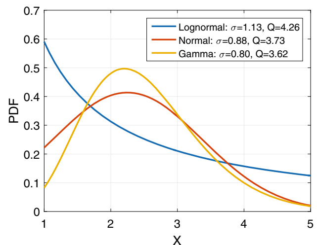
Fig. 1 Different continuous distributions with identical mean (2.5) which differ in other measures like standard deviation \sigma or 90 % quantiles Q
