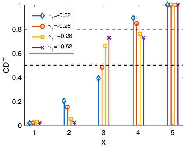
Fig. 2 Different discrete distributions with identical mean (3.5) and standard deviation (0.968). It can easily be seen that e.g. the median (and other important quantiles, in fact) are significantly different in each distribution
