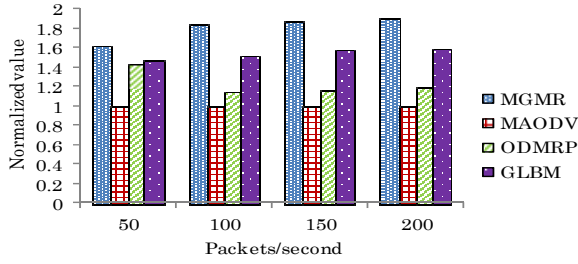
Fig. 13. Average packet delivery ratio in 100-nodes WCNs
