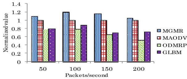
Fig. 14. Average throughput in 100-nodes WCNs
