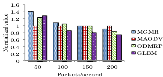
Fig. 10. Average throughput in 50-nodes WCNs
