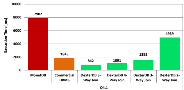
Figure 9: SSB Query 4.1 for Different Multi-Way/Star Join Configurations.
