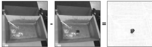
Figure 12: Grasp success is determined by subtracting images before an object is dropped into the bin (left) and after it was dropped (right).
