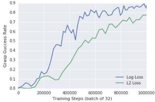
Figure 8: Loss function comparison in simulation
