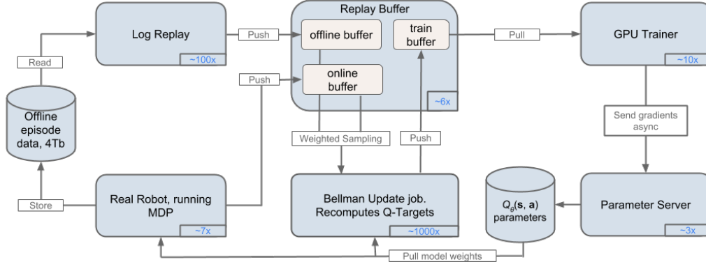
Figure 14: Architecture of the QT-Opt distributed reinforcement learning algorithm.
