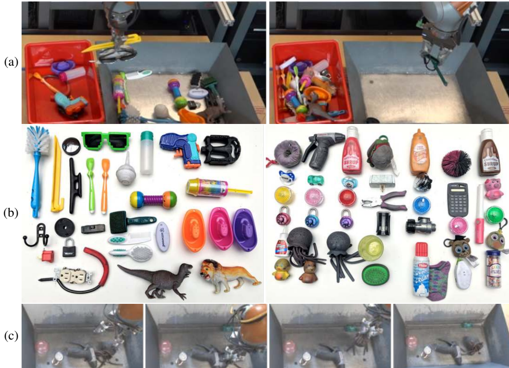
Figure 5: Illustrations of the bin emptying experiment (a). The (a, right) shows a very small object getting stuck in the corner and requiring a few attempts to get grasped. The test objects for the bin emptying experiment (b, left) and grasping with replacement experiment (b, right). Note that the objects range greatly in size and appearance, and many are exceedingly difficult to grasp due to small size, complex shapes, and varied material properties. Sequence (c) illustrates a grasp on the legs of a toy octopus, getting positive visual feedback and resulting in episode termination by the policy. During further ascent, the octopus slips out of the gripper, and the grasp is labeled as a failure. This is not a principled limitation of our method, as we could have terminated an episode at a larger height to get more robust feedback. Robot’s observation I_t is shown in (c).
