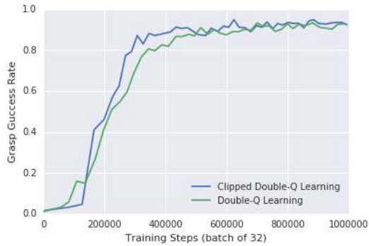
Figure 9: Comparison of DQN methods. See Appendix F.4 for clipped Double DQN definition.
