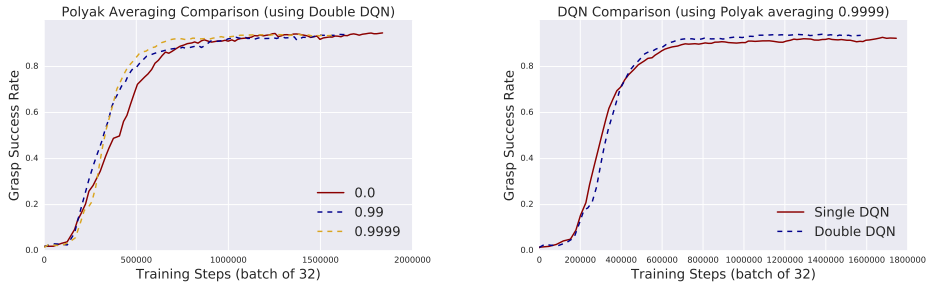
(a) All values of Polyak averaging provide stable training that reach similar performance, but higher values seem to converge faster and have smoother performance curves.
