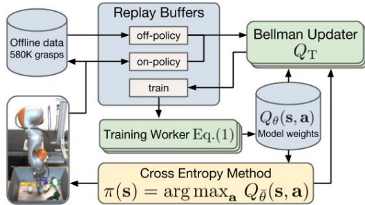
Figure 3: Our distributed RL infrastructure for QT-Opt (see Sec. 4.2). State-action-reward tuples are loaded from an offline data stored and pushed from online real robot collection (see Sec. 5). Bellman update jobs sample transitions and generate training examples, while training workers update the Q-function parameters.
