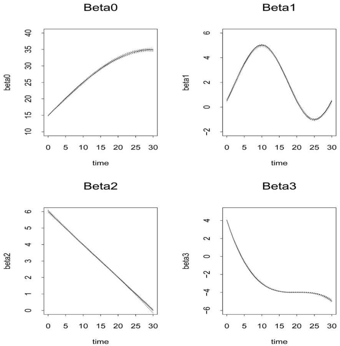
Figure 4. For continuous responses, fitted varying coefficient curves corresponding to 9 deciles of mean absolute deviation of errors from 1000 simulations. The solid lines are true coefficient curves.
