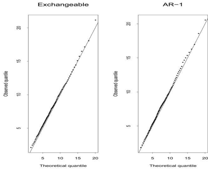
Figure 5. For continuous responses, quantile-quantile plots for test statistics Q(\tilde{\beta}) - Q(\hat{\beta}) versus \chi_8^2 under H_0 : \beta_1 is constant over time from 1000 simulations: (a) assume exchangeable working correlation; (b) assume AR-1 working correlation.
