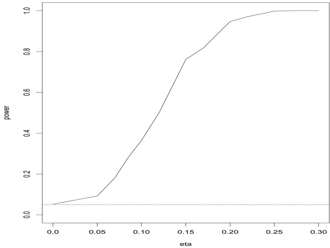
Figure 3. For binary responses, power of quadratic inference function against \eta for testing H_0: \beta_1 is constant over time, from 1000 simulations.
