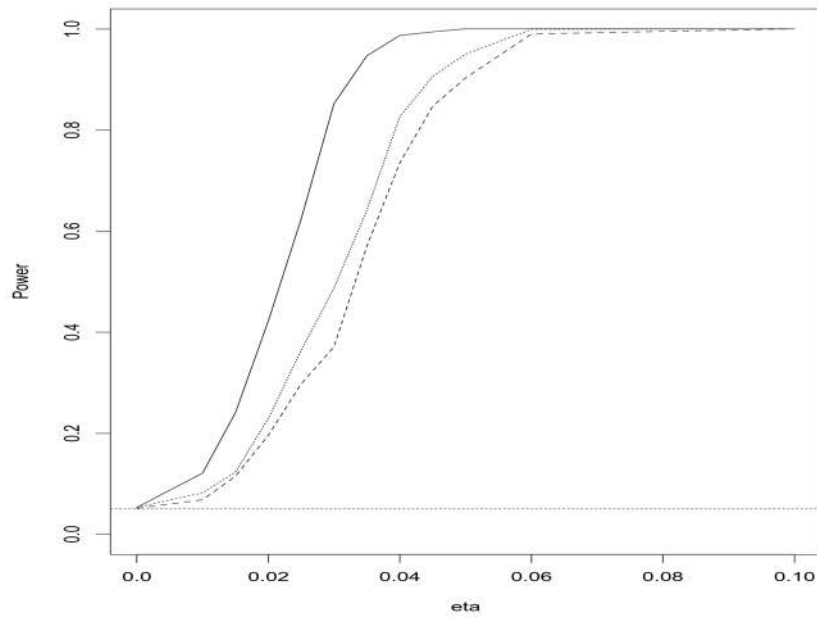
Figure 7. For continuous responses, power of quadratic inference function against \eta for testing H_0: \beta_1 is constant over time from 1000 simulations. The solid line is the power using exchangeable correlation, the dotted line is the power using AR-1 correlation and the dash line is the power using independent structure. The true correlation structure is exchangeable.
