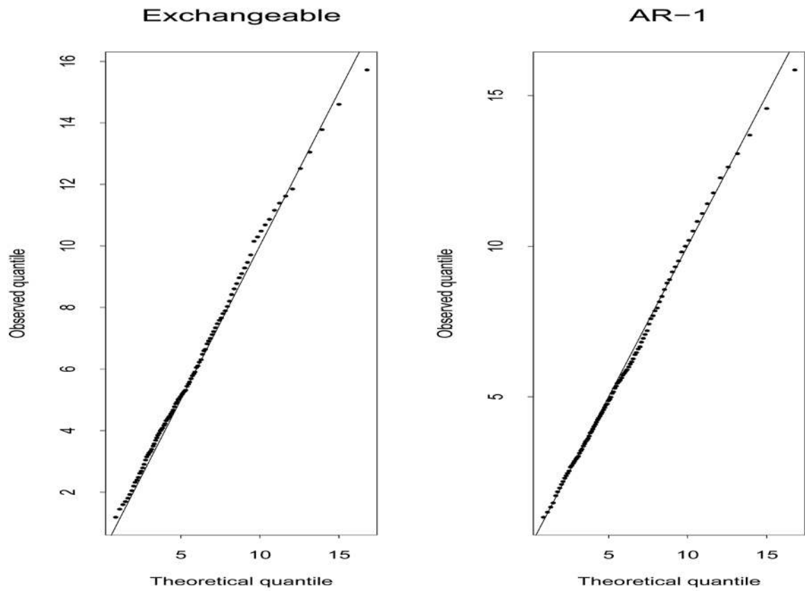
Figure 2. For binary responses, quantile-quantile plots for test statistics Q(\tilde{\beta}) - Q(\hat{\beta}) versus \chi_6^2 under H_0: \beta_1 is constant over time, from 1000 simulations: (a) assume exchangeable working correlation; (b) assume AR-1 working correlation.
