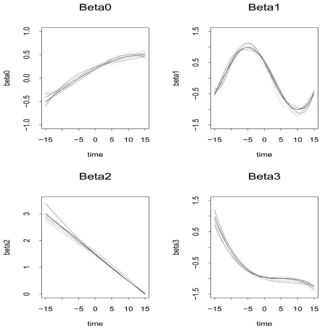
Figure 1. For binary responses, fitted varying coefficient curves corresponding to 9 deciles of mean absolute deviation of errors, from 1000 simulations. The solid lines are true coefficient curves.
