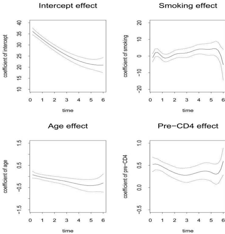
Figure 8. Fitted varying coefficients for AIDS data, where solid lines are fitted curves and dotted lines are 95% pointwise confidence intervals.
