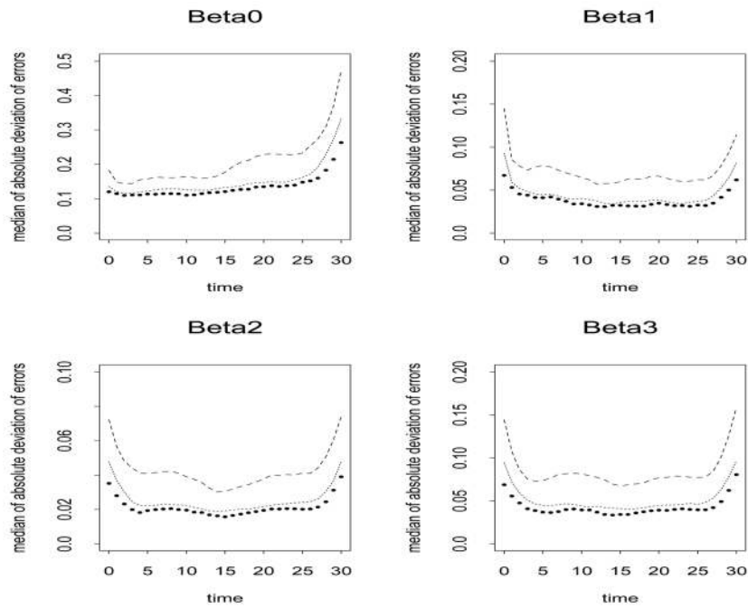
Figure 6. For continuous responses, the median of absolute deviation of errors between fitted and true values from 1000 simulations for three different working correlation structures. The bold dotted line is from exchangeable correlation, the dotted line is from AR-1 correlation and the dash line is from independent structure
