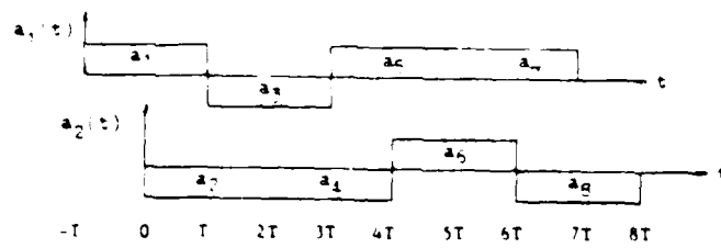
Staggering of data pulses in OQPSK
