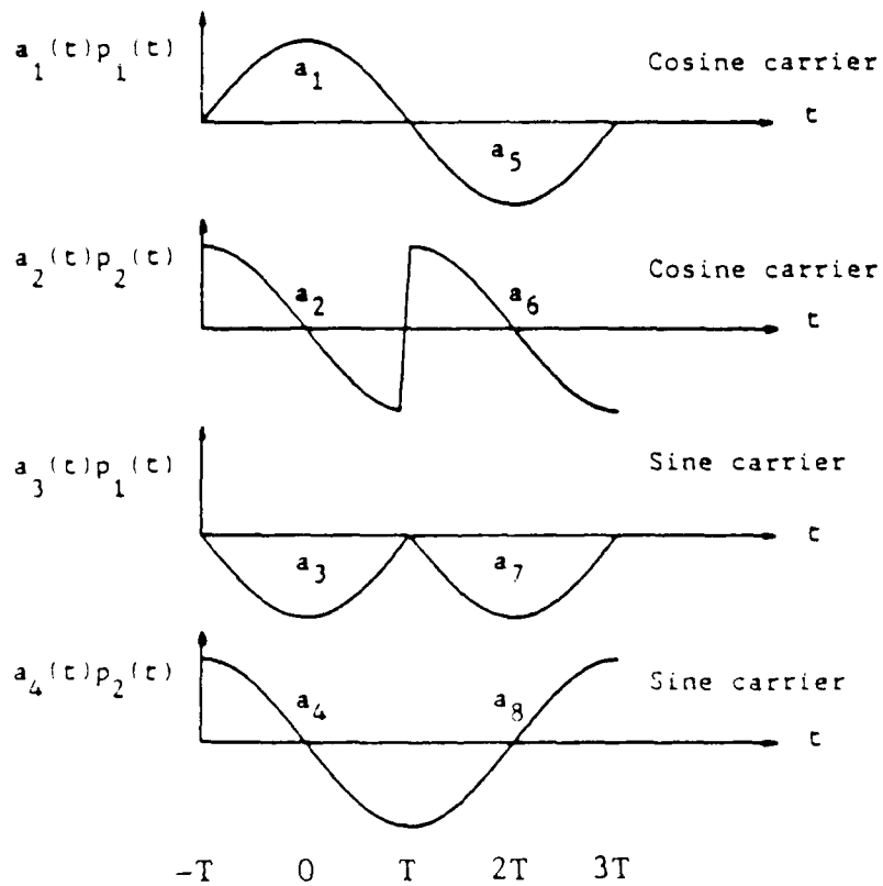
Figure 3.2. Wave shaping of the data pulses in Q^2PSK for the data stream a_4(t) in Figure 3.1.
