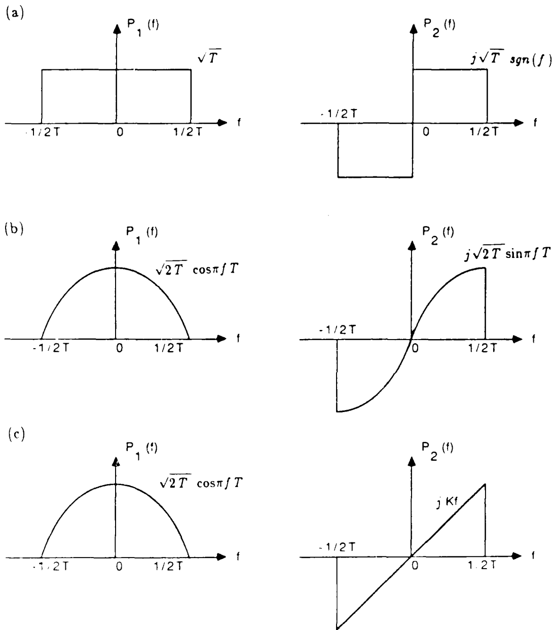
Figure 6.2. Transmitter filter pairs for Q^2PSK transmitter with zero inphase and zero cross intersymbol interference.
