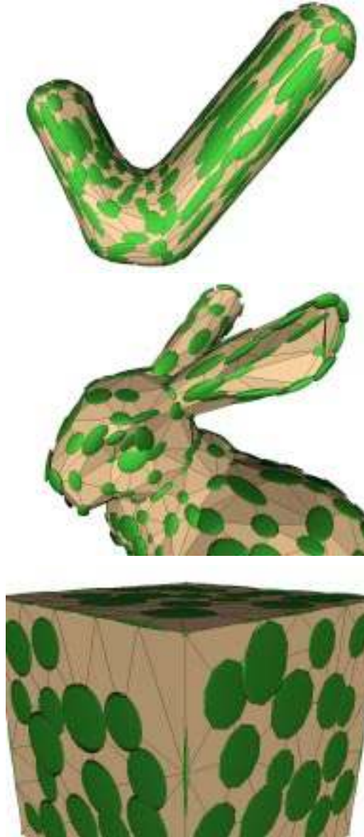
Figure 4.1: Quadric error isosurfaces on three simplified models: blobby “V”, bunny, and the corner of a cube. Note how the ellipsoids follow the local shape of each surface.
