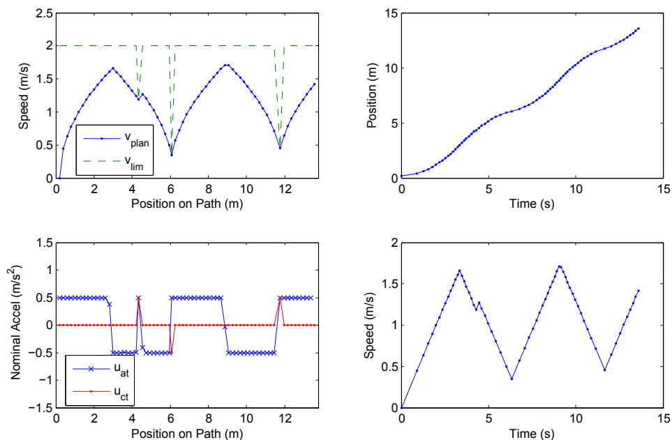
Figure 9. Results from optimizing the visibility graph based path, yielding a 13.6 sec plan. When the path changes direction around obstacle corners, the vehicle must slow down to a safe speed, accelerate laterally, then speed up again.
