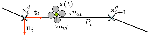
Figure 5. Vehicle path definition. While the quadrotor travels along segment P_i from waypoint \mathbf{x}_i^d to \mathbf{x}_{i+1}^d , it applies along track and cross track control inputs u_{at} and u_{ct} to follow the path segment.
