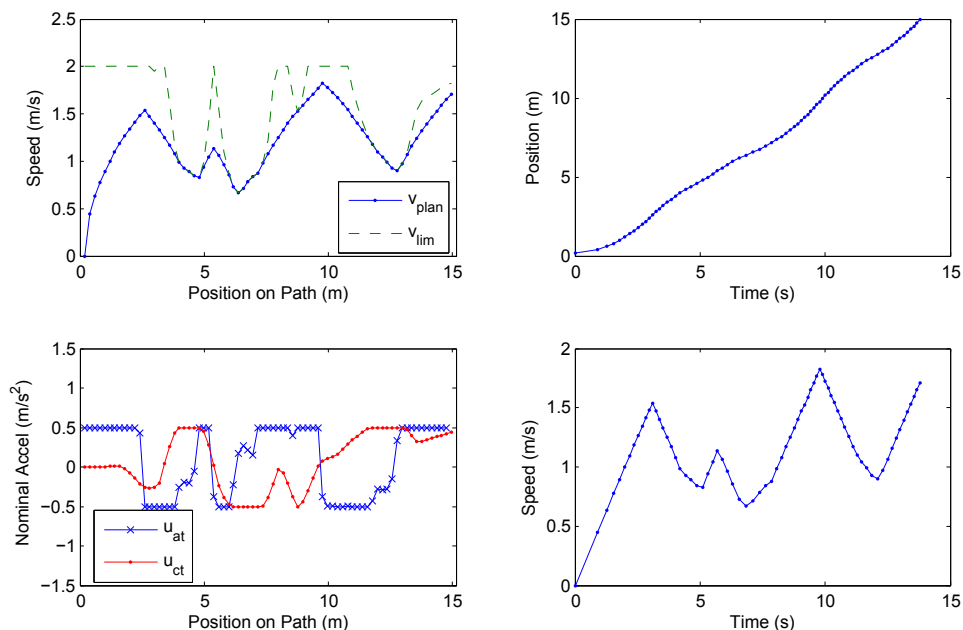
Figure 10. Results from optimizing the fast marching based path, yielding a 13.8 sec plan. Although this path is longer than the visibility graph based path, there are no corners, so the average speed is faster.
