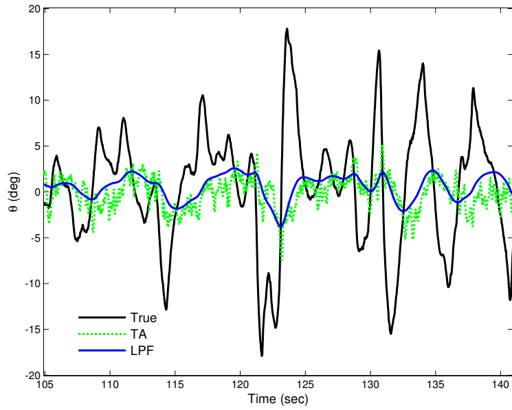
Figure 3: Pitch Angle Comparison. Comparison of the true pitch angle \theta , the traditional attitude approximation using only accelerometer information, and a low-pass filtered \theta for a small portion of a flight. Notice how closely the traditional attitude (TA) estimation method tracks the low-pass filtered pitch angle.
