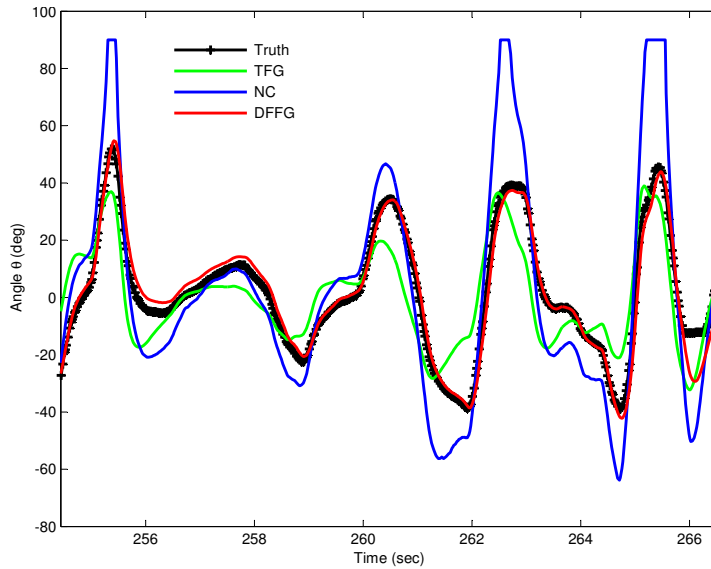
Figure 9: Pitch Angle During Aggressive Flight. This figure plots the true pitch angle \theta and its estimates using the traditional fixed-gain (TFG), nonlinear complementary (NC), and drag-force fixed-gain (DFFG) estimators during an aggressive flight. Notice that the DFFG provides accurate estimates despite the large angles that are experienced. The filter parameters are identical to those used to produce the previous plots. The saturation in the NC filter are due to the singularity at 90 degrees for a pitch angle. The NC filter was tuned to behave well for nominal flights, but the gains are inadequate for large pitch and roll maneuvers.
