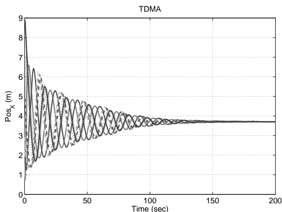
Fig. 10: Multi-agent consensus using TDMA
