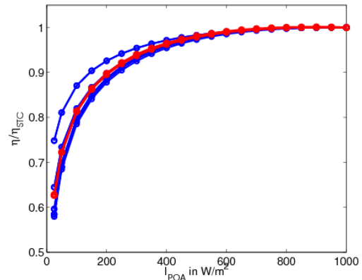
Figure 6: Normalized MPP efficiency curves ( 25^\circ\text{C} ) for a set of modules (blue lines) and the representative efficiency curve (red lines) reflecting the average efficiency values at non STC-irradiances.
