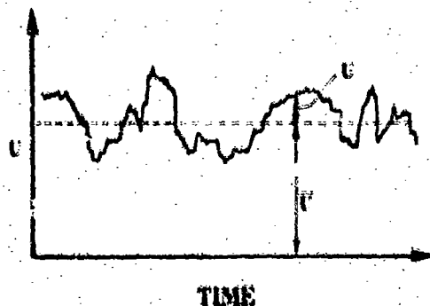
Figure 6.2. Windspeed showing effects of turbulence (Pasquill, 1974).
