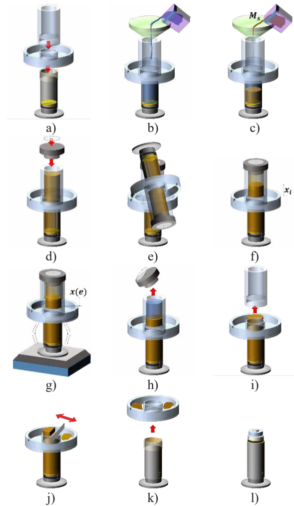
Fig. 5. Schematic procedure of specimen reconstitution.
