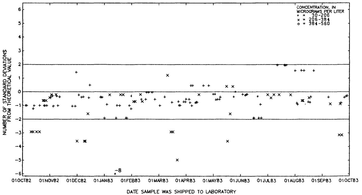
Figure 10.--Barium, dissolved, data from the Denver laboratory.
