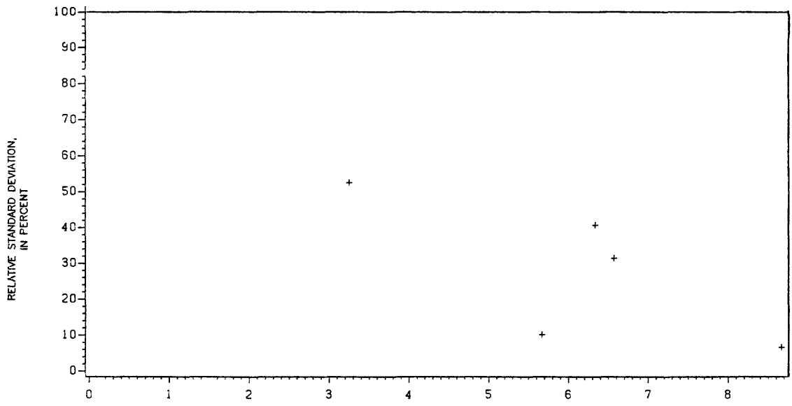
MEAN CONCENTRATION, IN MICROGRAMS PER LITER Figure 165.-- Precision data for silver, total recoverable, at the Atlanta laboratory.
