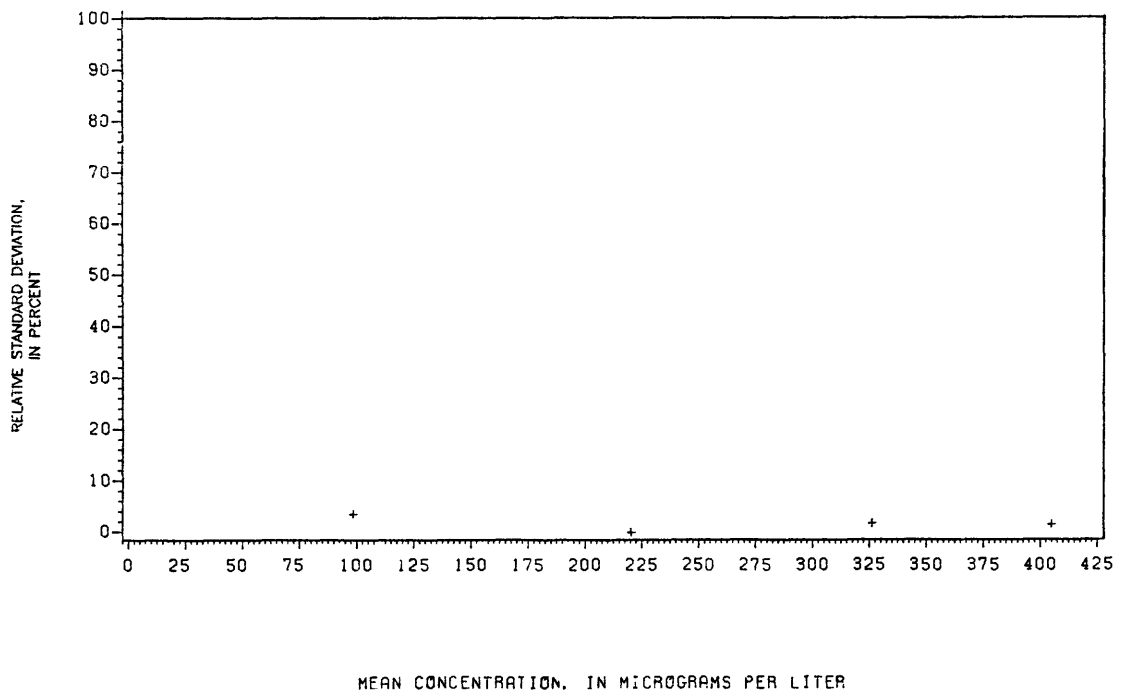
Figure 150.-- Precision data for manganese, total recoverable, at the Denver laboratory.
