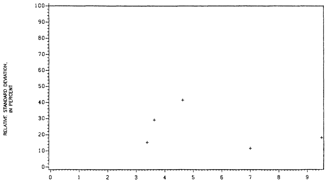
MEAN CONCENTRATION, IN MICROGRAMS PER LITER Figure 166.-- Precision data for silver, total recoverable, at the Denver laboratory.
