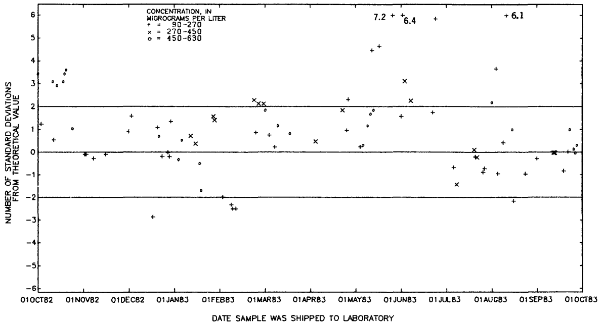
Figure 3.--Aluminum, dissolved, data from the Atlanta laboratory.
