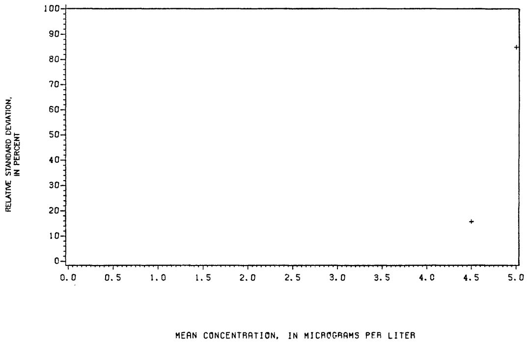
Figure 95.-- Precision data for antimony, dissolved, at the Atlanta laboratory.
