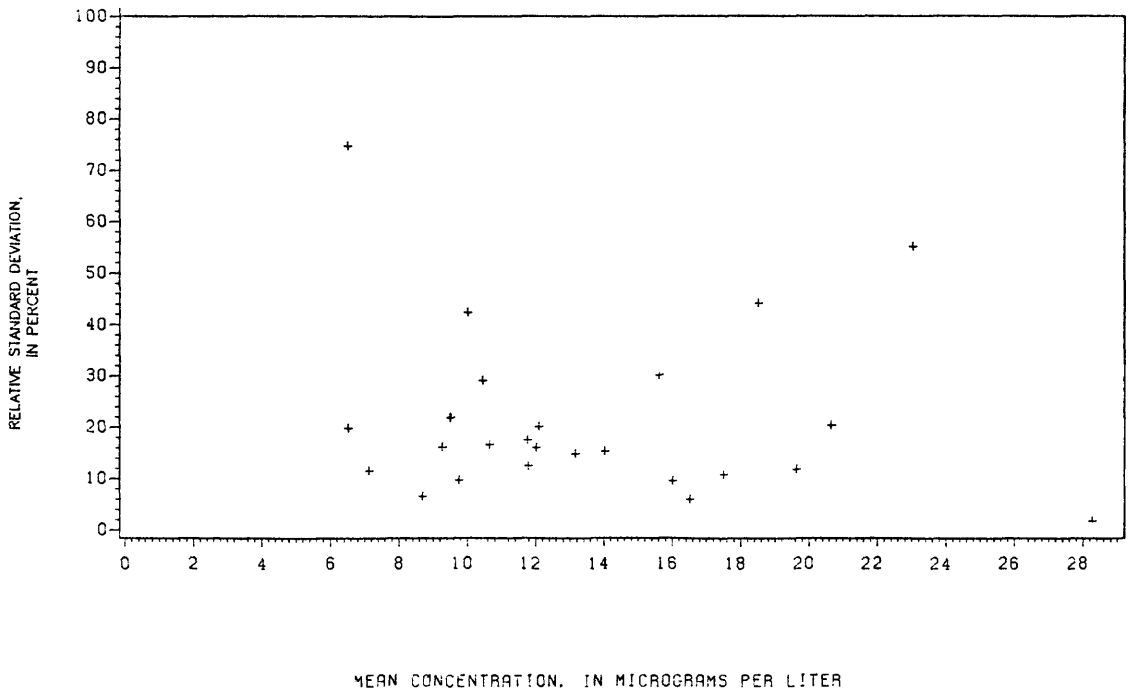
Figure 154.-- Precision data for nickel, dissolved, at the Denver laboratory.
