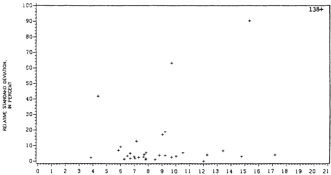
MEAN CONCENTRATION, IN MILLIGRAMS PER LITER Figure 162.-- Precision data for silica, dissolved, at the Denver laboratory.
