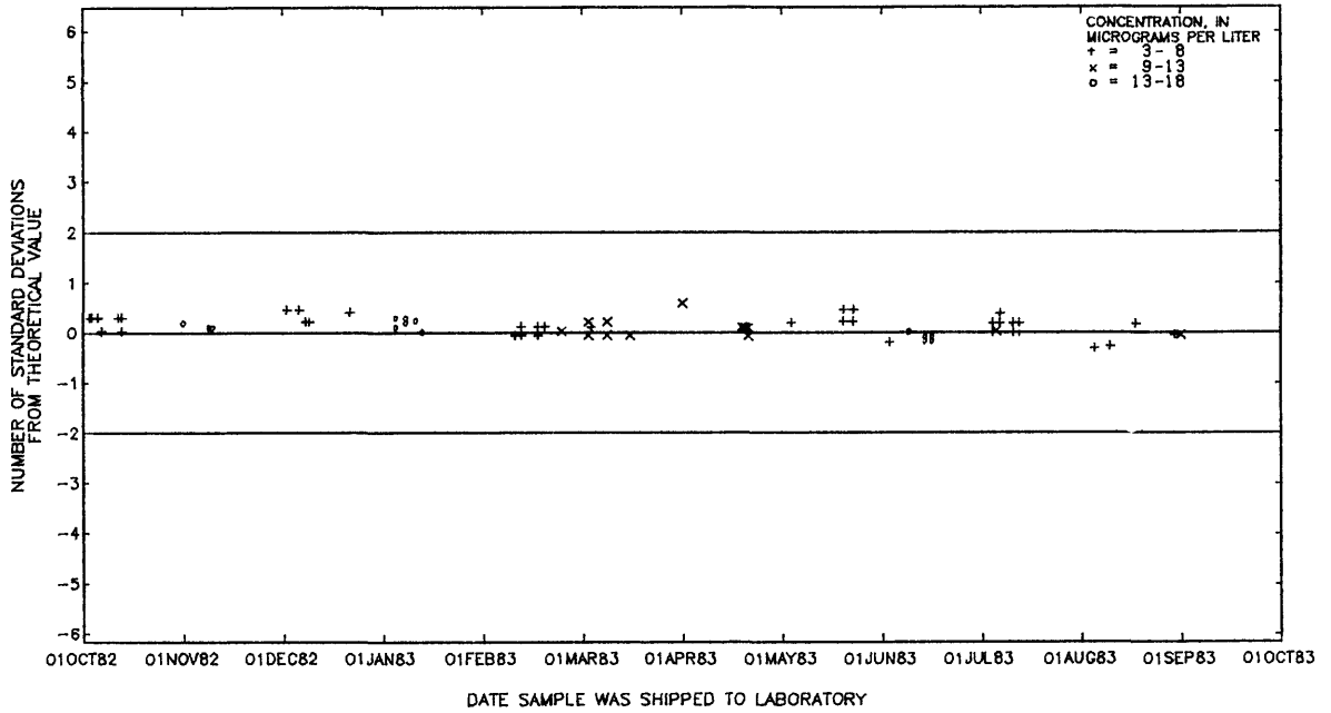
Figure 69.--Selenium, dissolved, data from the Atlanta laboratory.
