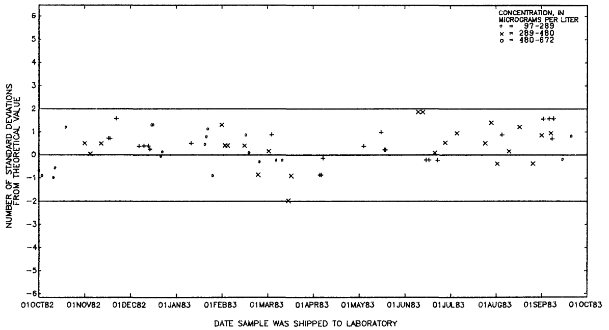
Figure 83.--Strontium, dissolved, data from the Atlanta laboratory.
