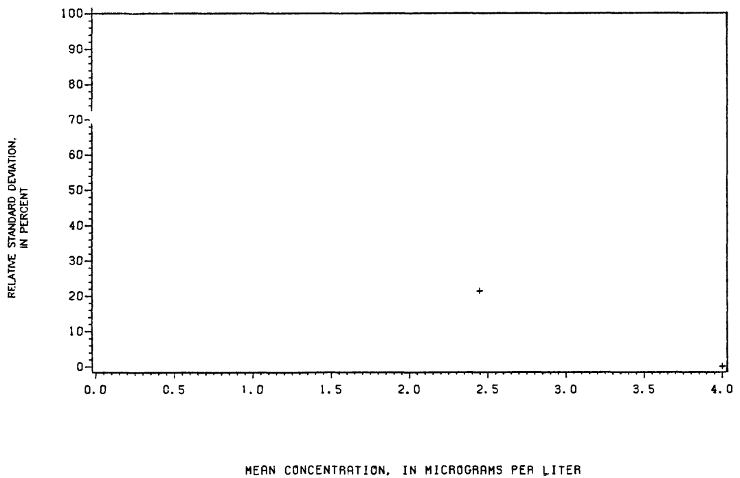
Figure 96.-- Precision data for antimony, dissolved, at the Denver laboratory.
