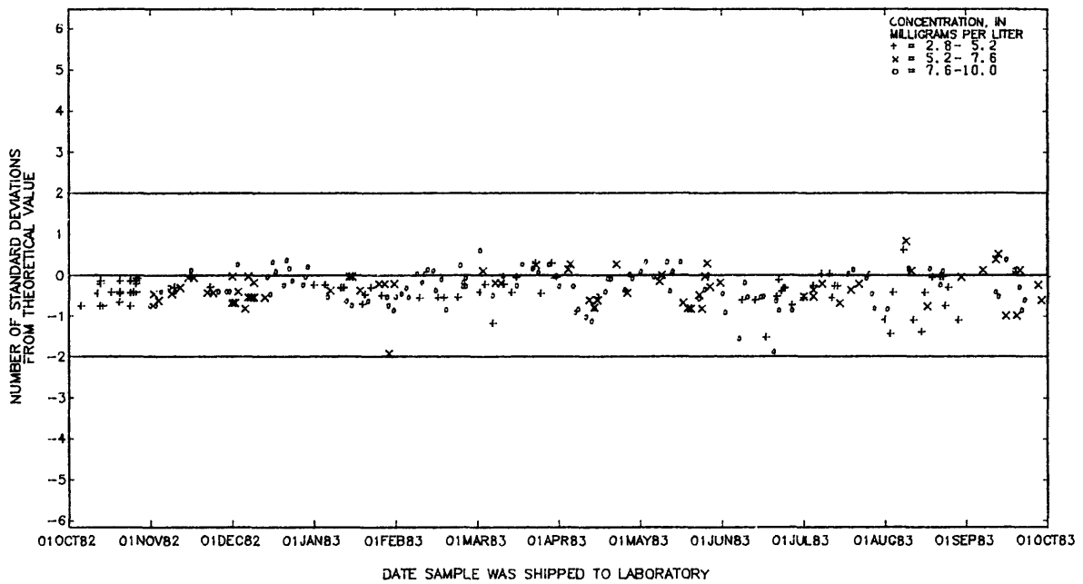
Figure 68.--Potassium, dissolved, data from the Denver laboratory.
