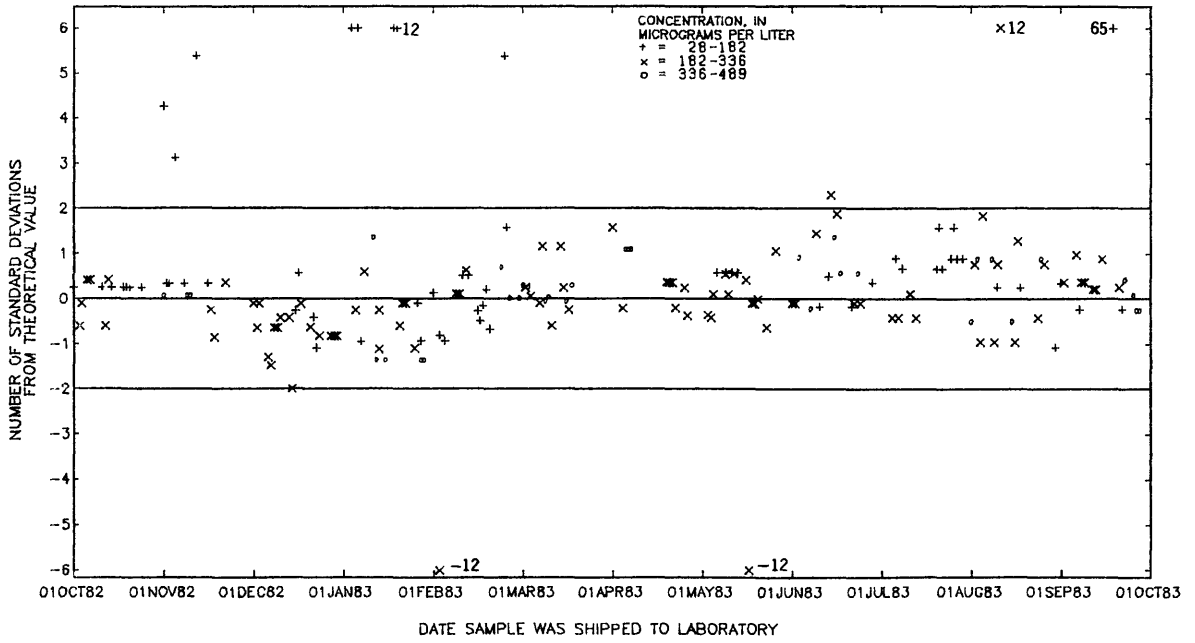
Figure 87.--Zinc, dissolved, data from the Atlanta laboratory.
