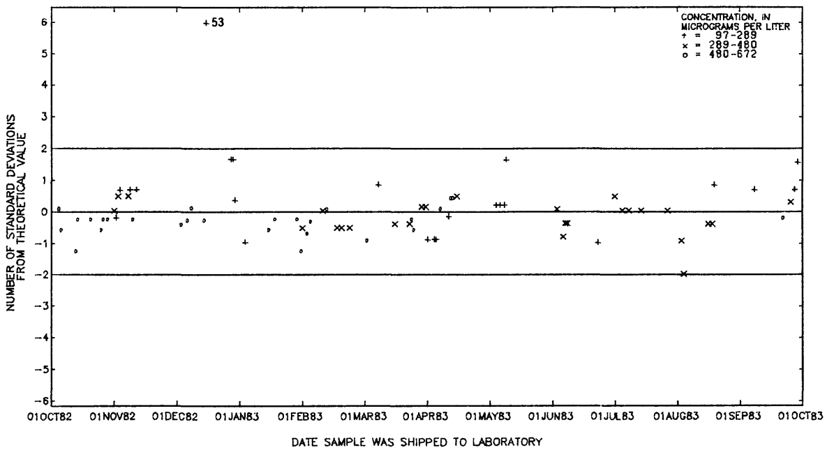
Figure 84.--Strontium, dissolved, data from the Denver laboratory.
