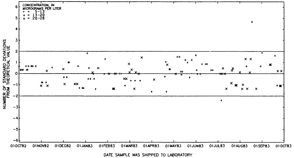
Figure 27.--Chromium, dissolved, data from the Atlanta laboratory.
