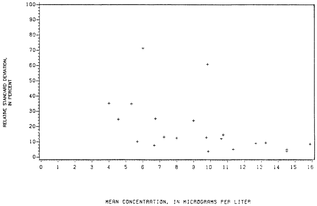
Figure 121.-- Precision data for cobalt, dissolved, at the Atlantic laboratory.
