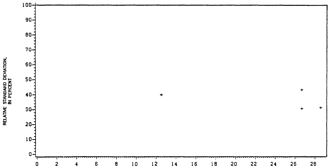
MEAN CONCENTRATION, IN MICROGRAMS PER LITER Figure 119.— Precision data for chromium, total recoverable, at the Atlanta laboratory.
