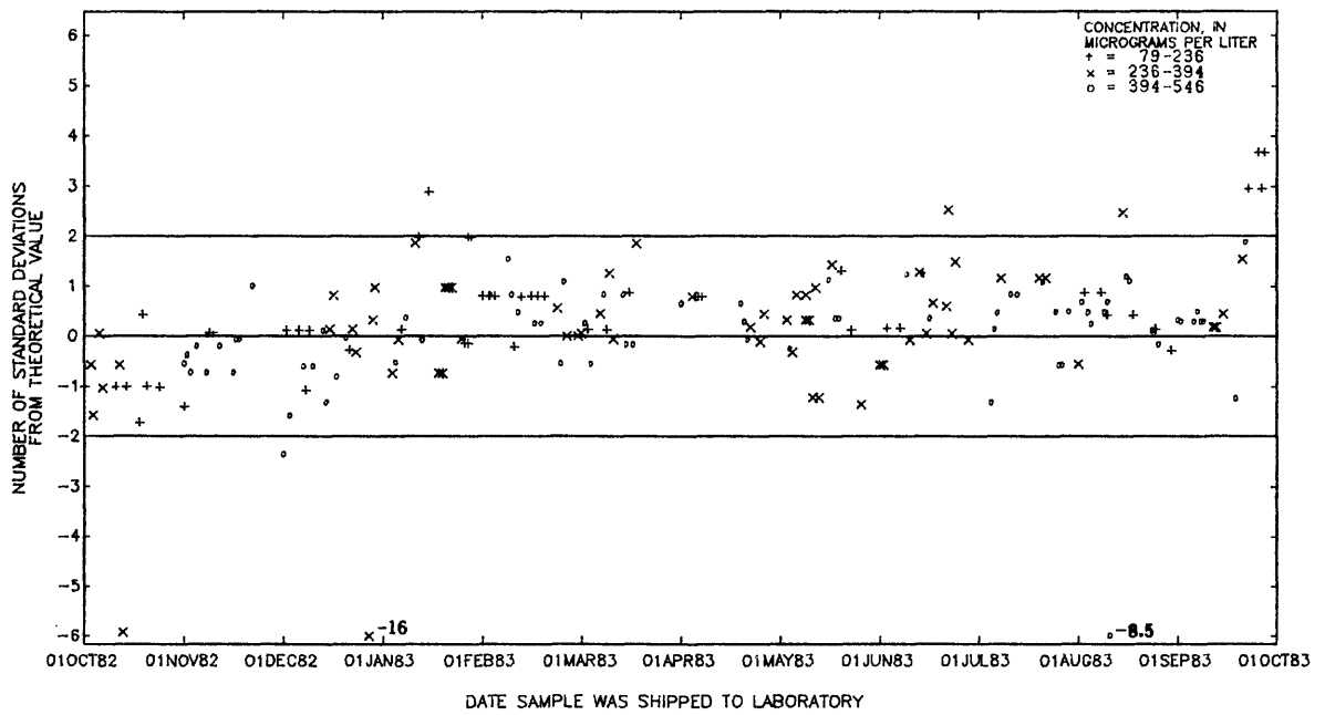
Figure 57.--Manganese, dissolved, data from the Atlanta laboratory.
