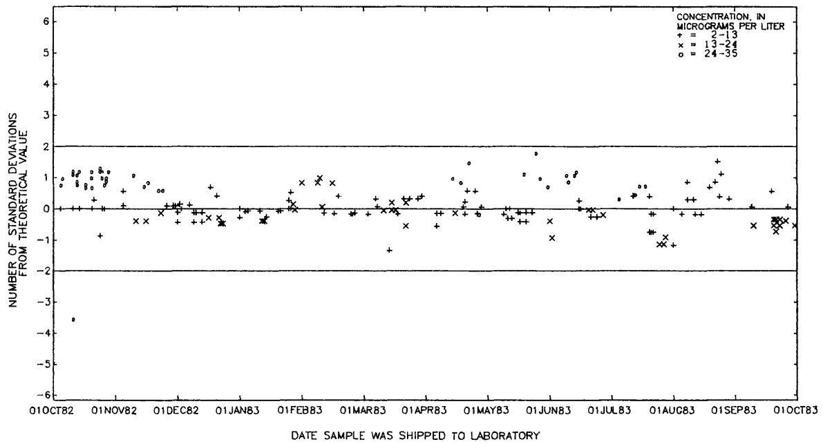
Figure 8.--Arsenic, dissolved, data from the Denver laboratory.
