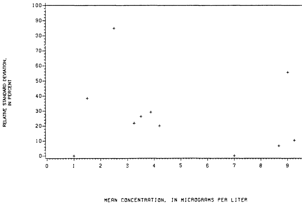
Figure 164.-- Precision data for silver, dissolved, at the Denver laboratory.
