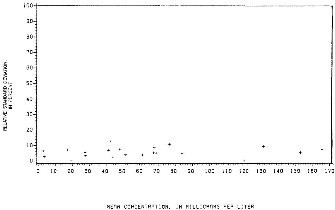
MEAN CONCENTRATION, IN MILLIGRAMS PER LITER Figure 167.-- Precision data for sodium, dissolved (inductively coupled plasma emission spectrometry), at the Atlanta laboratory.
