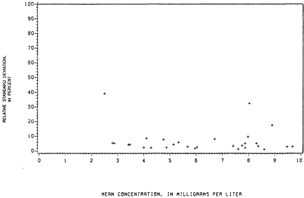
Figure 157.-- Precision data for potassium, dissolved, at the Atlanta laboratory.
