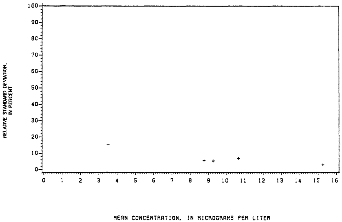
Figure 110.— Precision data for cadmium, total recoverable, at the Denver laboratory.
