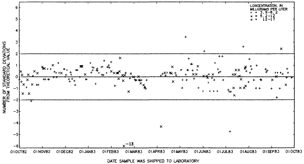
Figure 71.--Silica, dissolved, data from the Atlanta laboratory.
