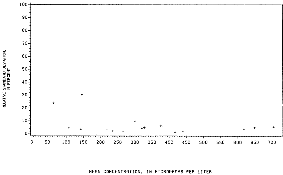
Figure 94.-- Precision data for aluminum, dissolved, at the Denver laboratory.
