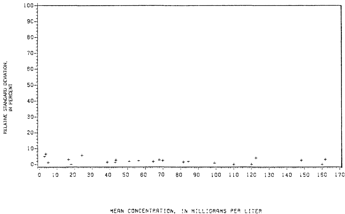
MEAN CONCENTRATION, IN MILLIGRAMS PER LITER Figure 168.-- Precision data for sodium, dissolved (inductively coupled plasma emission spectrometry), at the Denver laboratory.
