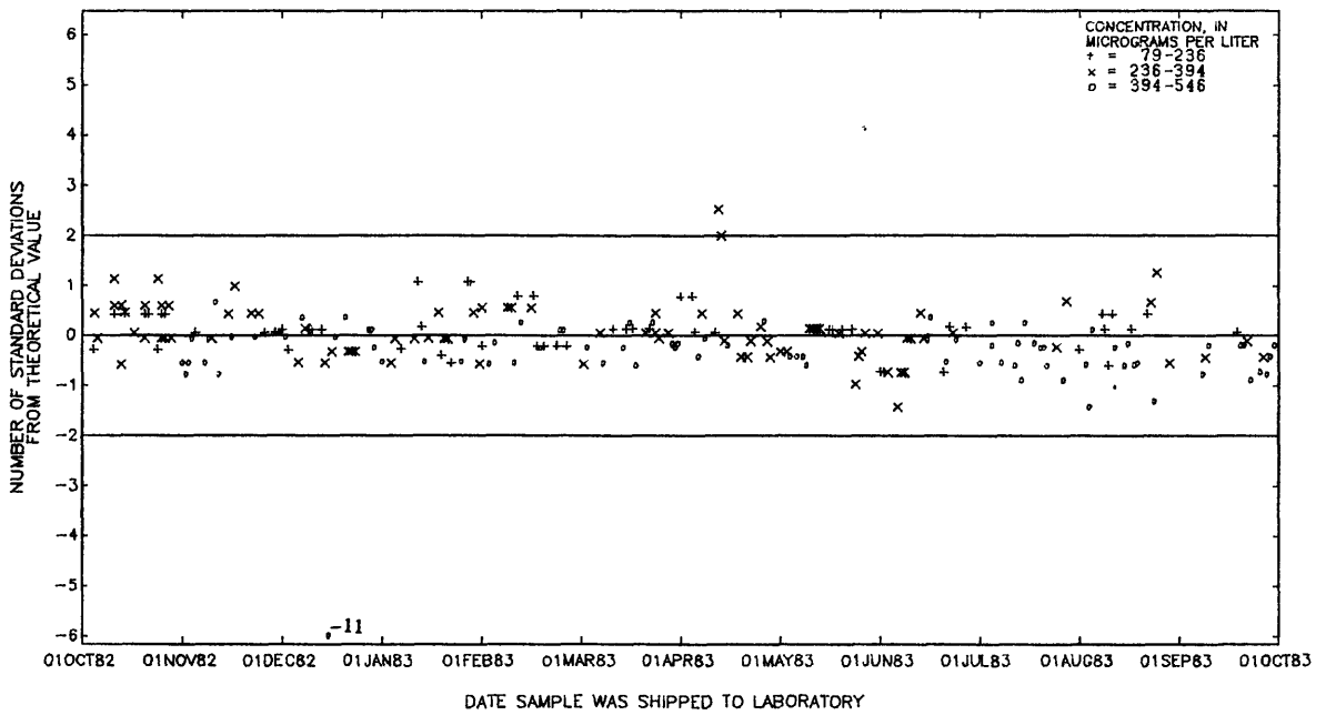
Figure 58.--Manganese, dissolved, data from the Denver laboratory.
