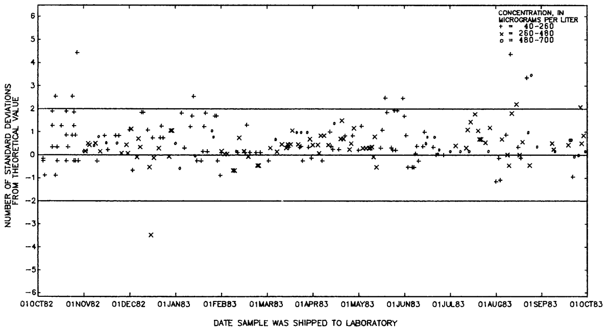
Figure 44.--Iron, dissolved, data from the Denver laboratory.
