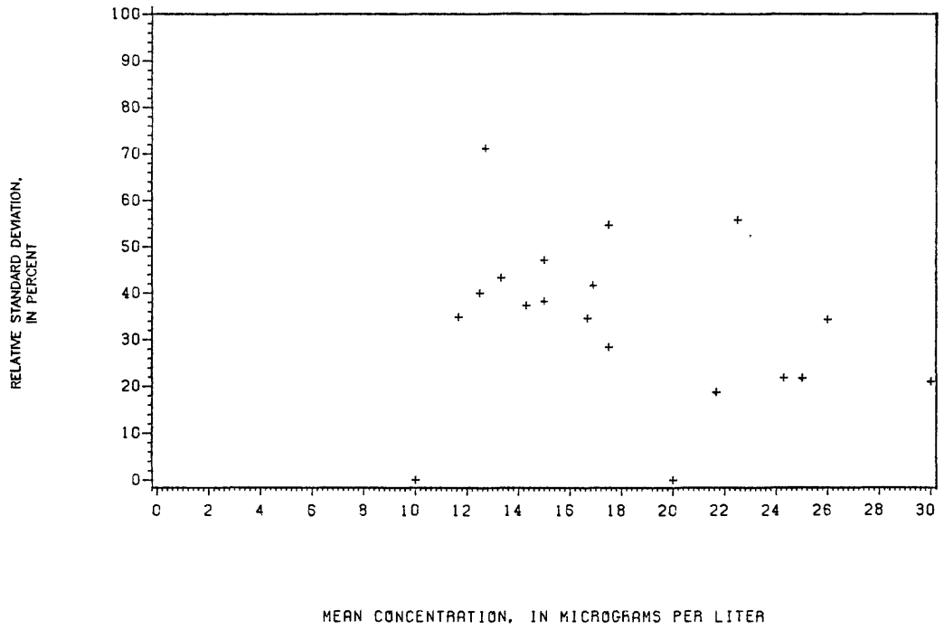
Figure 117.-- Precision data for chromium, dissolved, at the Atlanta laboratory.
