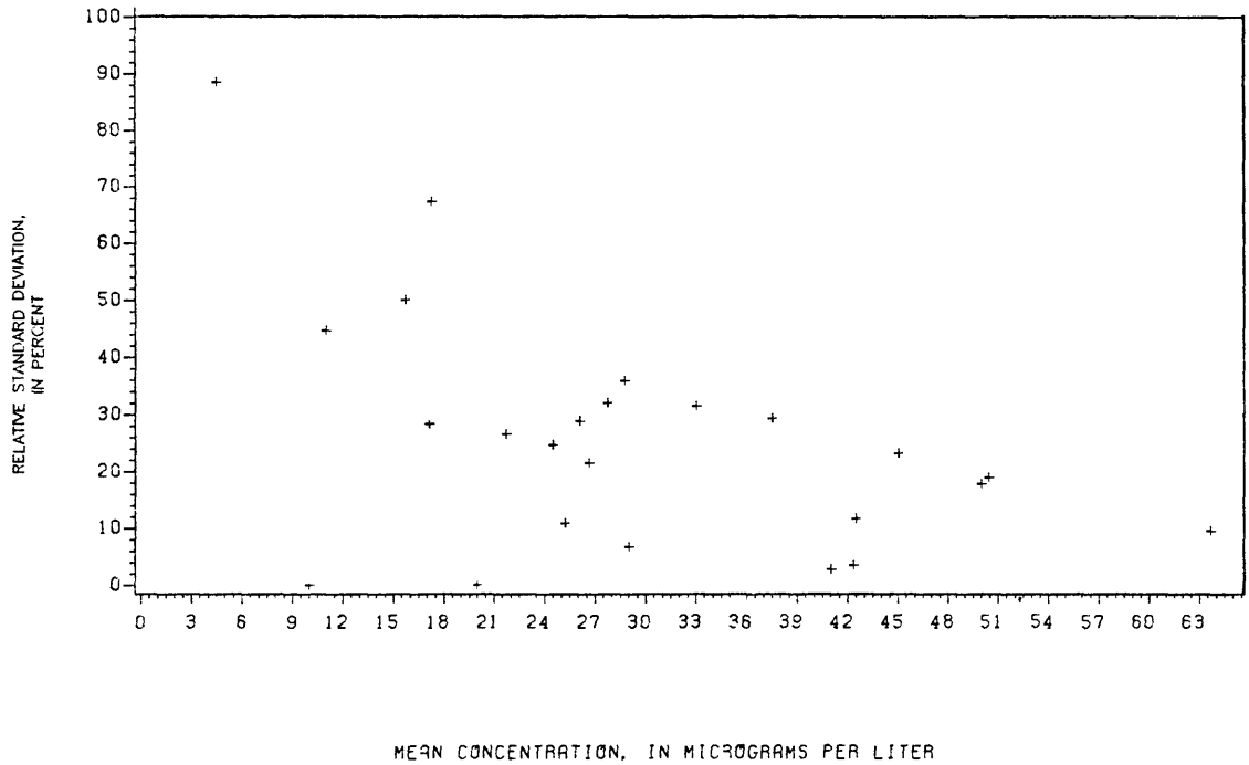
Figure 151.-- Precision data for molybdenum, dissolved, at the Atlanta laboratory.
