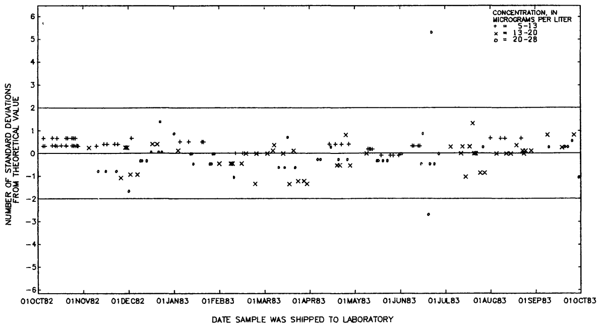
Figure 28.--Chromium, dissolved, data from the Denver laboratory.
