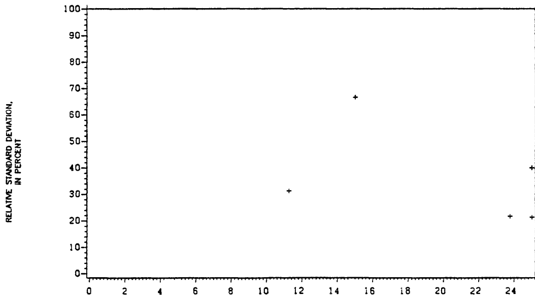
MEAN CONCENTRATION, IN MICROGRAMS PER LITER Figure 120.— Precision data for chromium, total recoverable, at the Denver laboratory.
