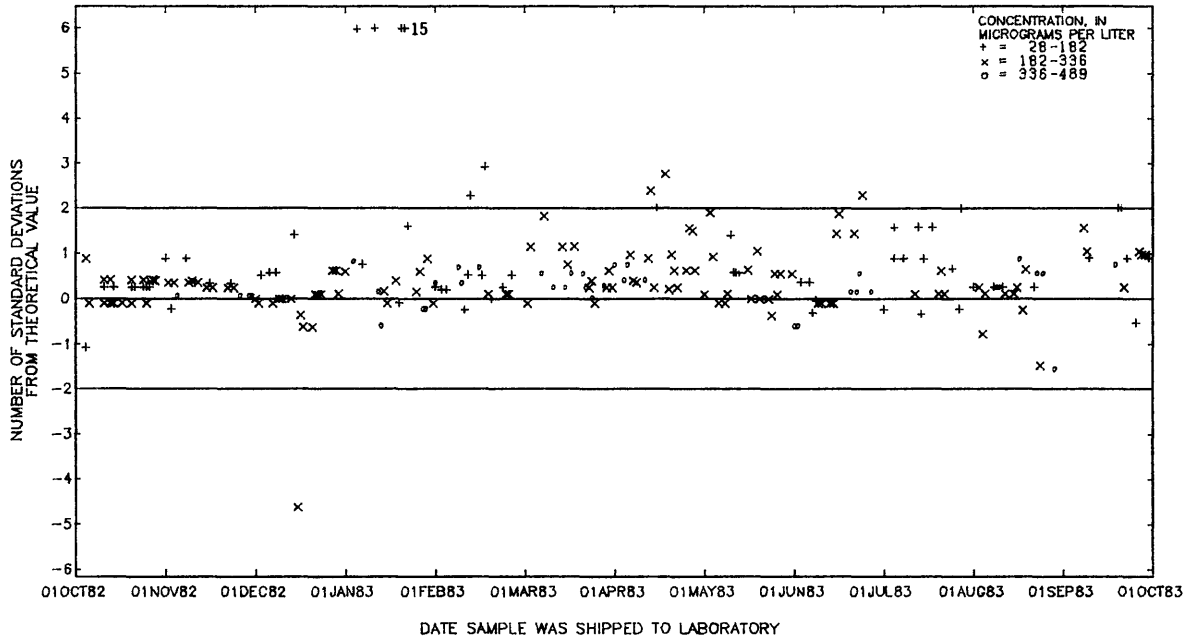
Figure 88.--Zinc, dissolved, data from the Denver laboratory.
