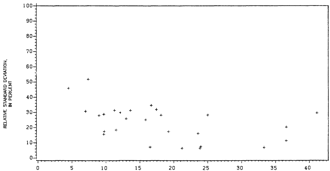
MEAN CONCENTRATION, IN MICROGRAMS PER LITER Figure 138.— Precision data for lead, dissolved, at the Denver laboratory.
