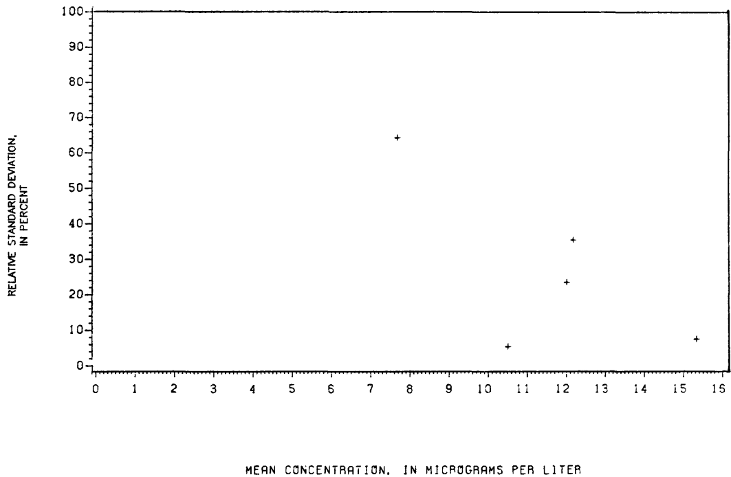
Figure 155.— Precision data for nickel, total recoverable, at the Atlanta laboratory.
