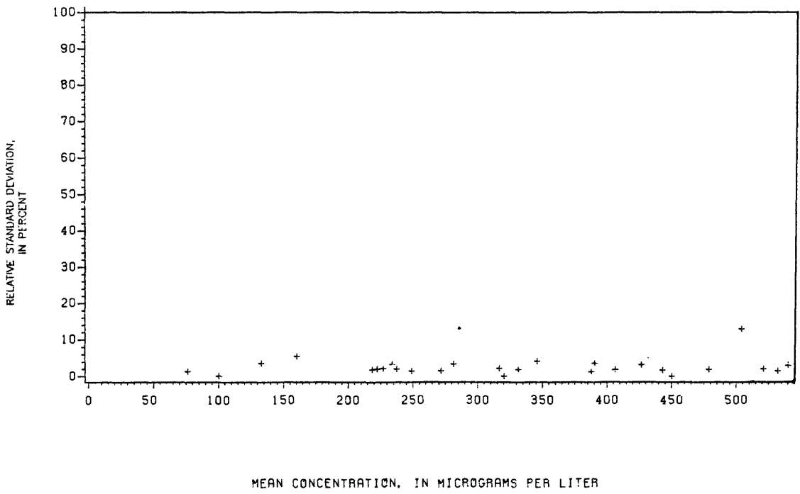
Figure 148.-- Precision data for manganese, dissolved, at the Denver laboratory.
