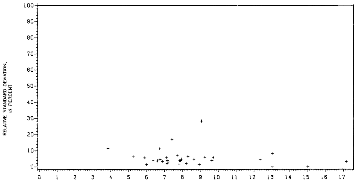
MEAN CONCENTRATION, IN MILLIGRAMS PER LITER Figure 161.-- Precision data for silica, dissolved, at the Atlanta laboratory.
