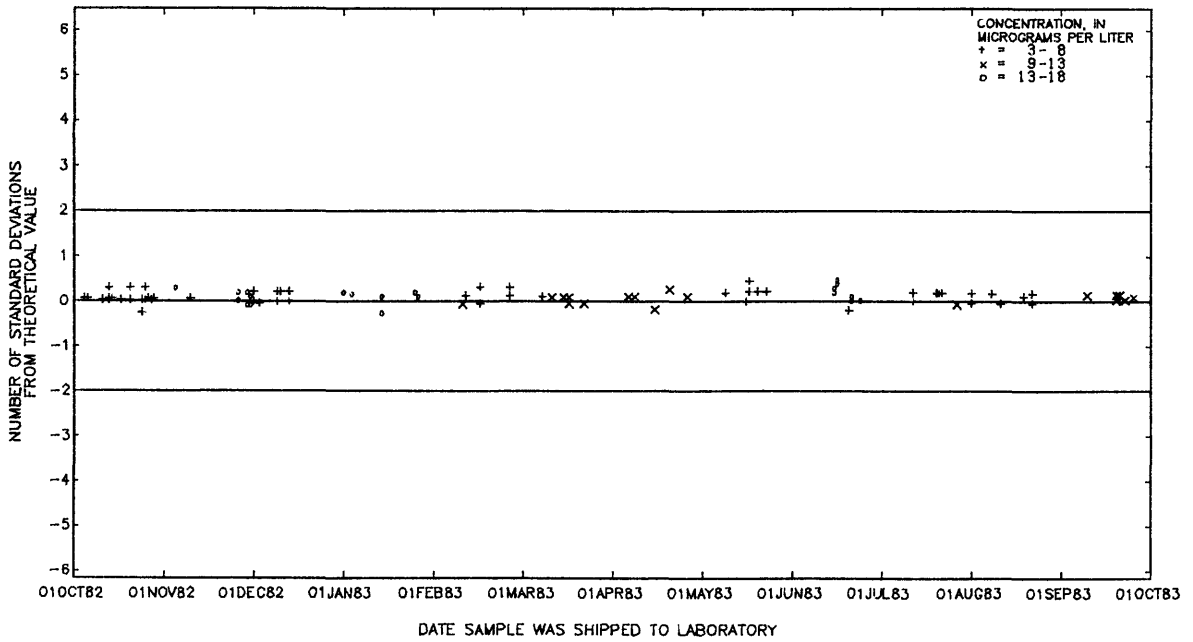
Figure 70.--Selenium, dissolved, data from the Denver laboratory.
