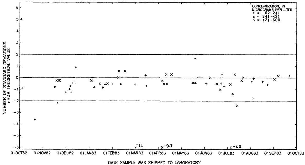
Figure 15.--Boron, dissolved, data from the Atlanta laboratory.
