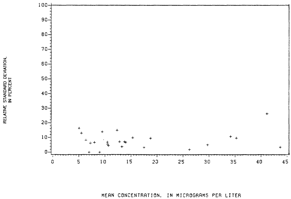
Figure 98.-- Precision data for arsenic, dissolved, at the Denver laboratory.
