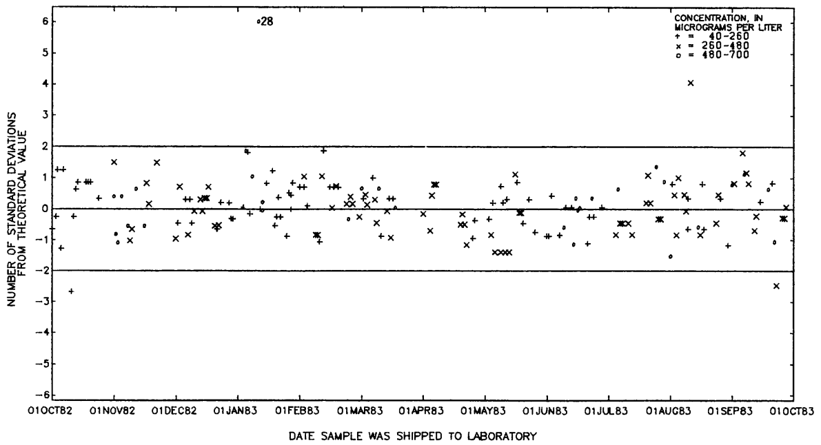
Figure 43.--Iron, dissolved, data from the Atlanta laboratory.
