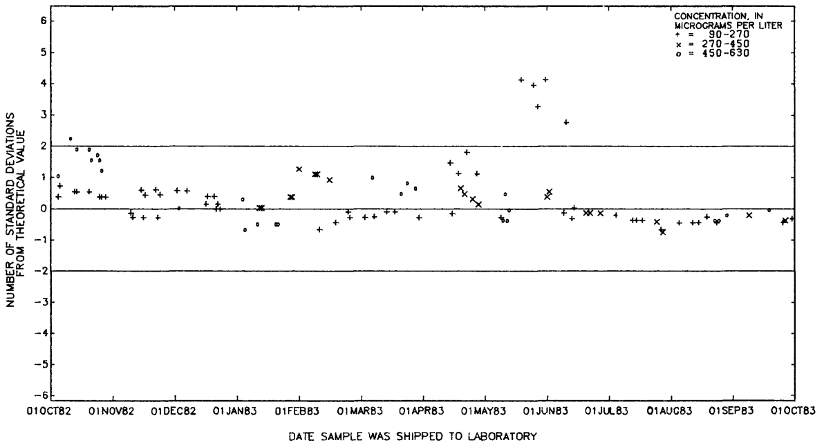
Figure 4.--Aluminum, dissolved, data from the Denver laboratory.
