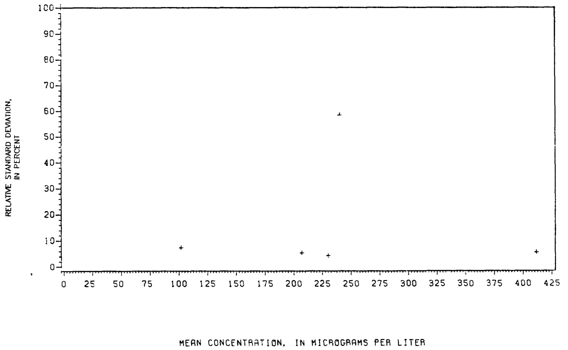
Figure 149.-- Precision data for manganese, total recoverable, at the Atlanta laboratory.
