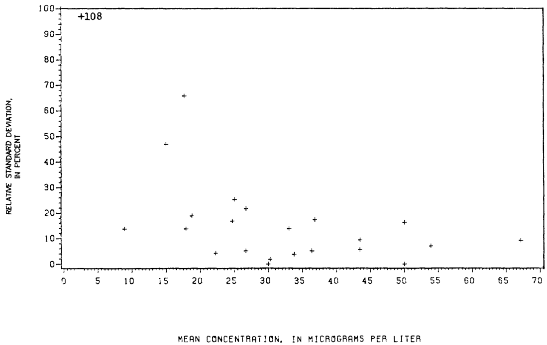
Figure 152.-- Precision data for molybdenum, dissolved, at the Denver laboratory.
