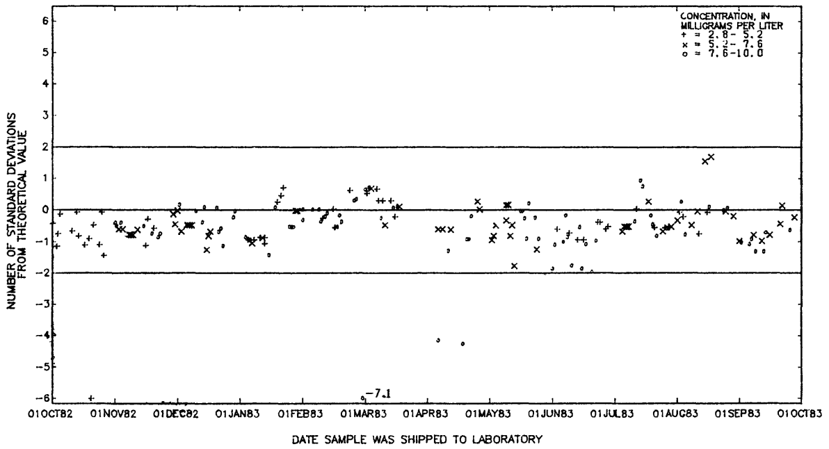
Figure 67.--Potassium, dissolved, data from the Atlanta laboratory.
