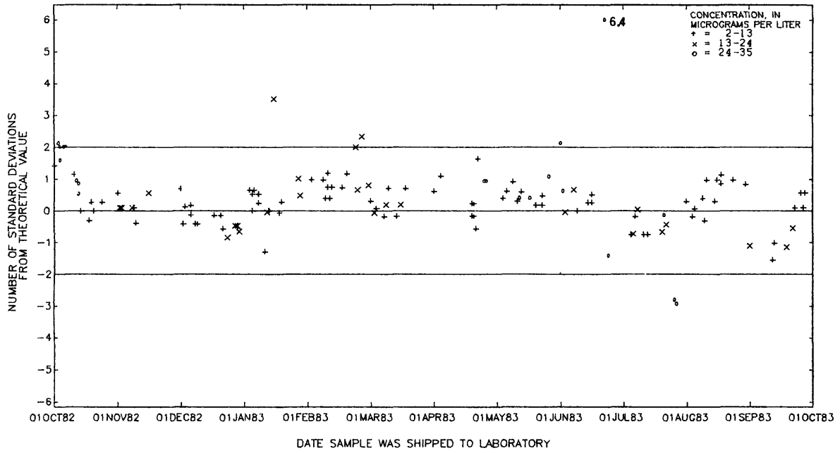
Figure 7.--Arsenic, dissolved, data from the Atlanta laboratory.
