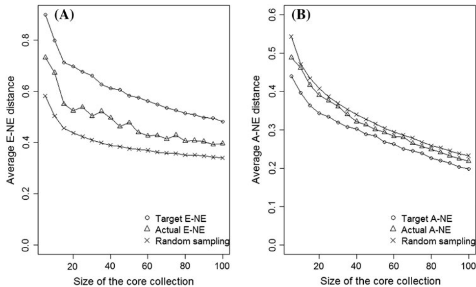
Fig. 9 Plot of average distance between an entry and the nearest neighbouring entry (E-NE) (a) and average distance between each accessions and its nearest entry in the core (A-NE) (b) against the size of core collection for bean data set. The bean data set was split into two halves with one half used to form collection and the other half used for evaluation of the core. Target (E-NE and A-NE) values
