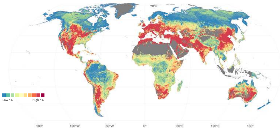
MAP 1.2: Global Risk of Poor Water Quality
