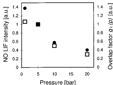
Fig. 4. Comparison of measured NO LIF intensities (on a relative scale, open squares) with calculated overlap factors g_\lambda(p) (filled circles) versus pressure. Both data series are on a relative scale and are scaled to overlap at 5 bars.
