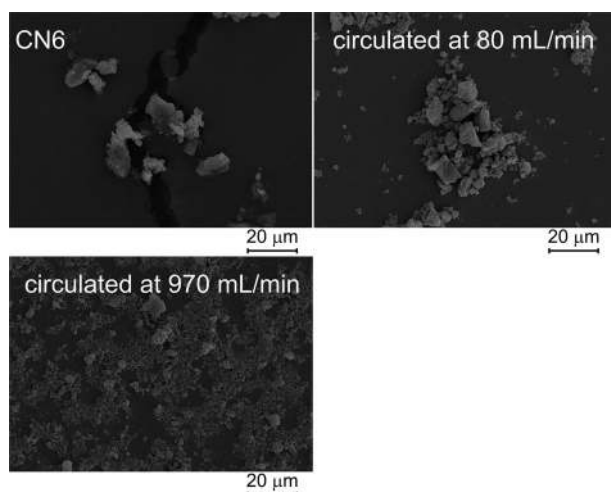
Fig. 5 SEM pictures of the photocatalyst before (upper left), after circulation at 80 mL \text{min}^{-1} (upper right) and after circulation at 970 mL \text{min}^{-1} (lower left).
