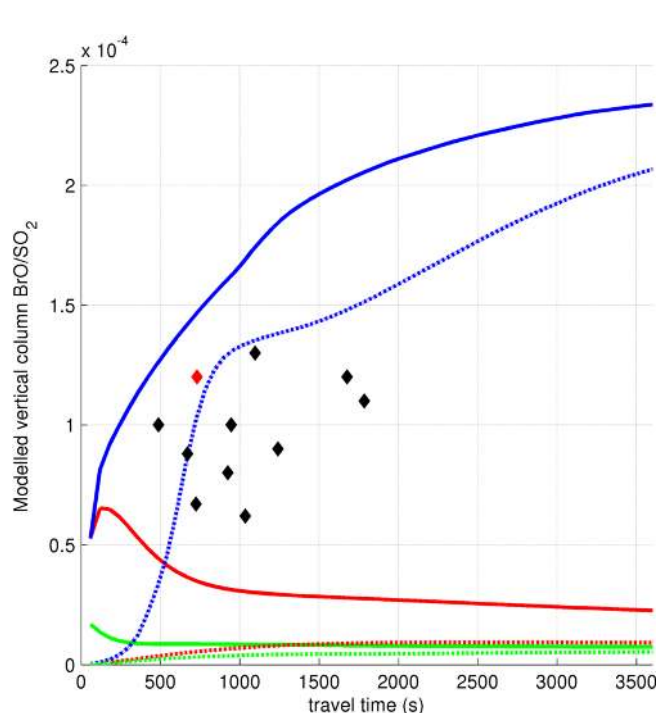
Figure 11. Evolution of vertical column BrO / \text{SO}_2 ratios for the six model scenarios discussed in the text (“low Br / S” initialisation). The colour code is the same as in Fig. 7. The black diamonds represent the spectroscopic measurements listed in Table 5, the red diamond represents the 2012-07-27 measurement contemporaneous with near-crater measurements of both \text{O}_3 and \text{SO}_2 .
