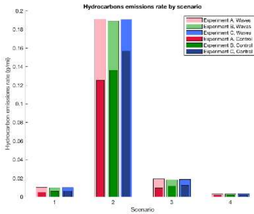
(a) Hydrocarbon emissions rate.
