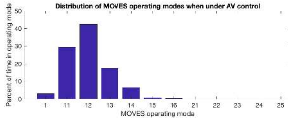
(c) Distribution of MOVES operating modes in Experiment C.
