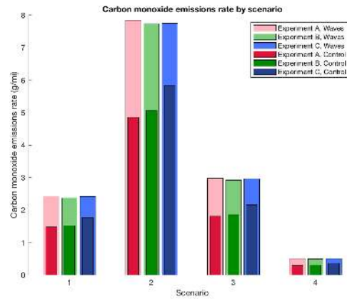
(b) Carbon monoxide emissions rate.
