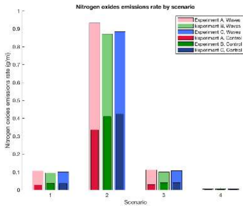
(c) Nitrogen oxides emissions rate.
