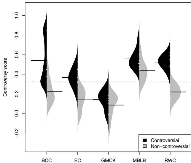
Figure 4: Controversy scores on follow graphs of various controversial and non-controversial datasets.
