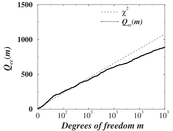
Fig. 2. Cross-correlations between the differences of logarithms of prices for IBM and General Electric (GE). We show Q_{CC}(m) versus the degrees of freedom m . We also show the critical values for the \chi^2(m) distribution at the 5% level of significance. Q_{CC}(m) virtually follows the critical values for the \chi^2(m) distribution that is a signal for no cross-correlations. The test of equation (7) gives practically the same result as the test of equation (6) since N \gg 1 .
