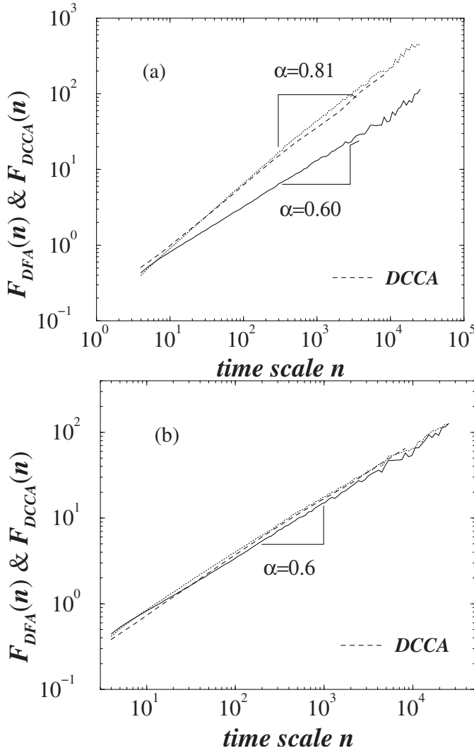
Fig. 4. DFA and DCCA scaling functions F_{DFA}(n) and F_{DCCA}(n) , respectively, versus time scale n . We generate the time series \{y_i\} and \{y'_i\} defined by the two-component process of equations (2a, 2b) with \rho_1 = 0.4 and \rho_2 = 0.1 . We exclude the sinusoidal amplitude, so A_1 = A_2 = 0 . We show the two DFA functions, F_{DFA}(n) \propto n^{\lambda_{DFA}} , and the DCCA function, F_{DCCA}(n) \propto n^{\lambda_{DCCA}} , for (a) W = 0.95 and (b) W = 0.5 . The closer W is to 0.5, the more the two processes y_i and y'_i become alike. \lambda_{DCCA} gradually decreases toward \lambda_{DFA} \approx 0.6 . Generally, by varying W , \lambda_{DCCA} becomes closer to \lambda_{DFA} corresponding to y_i , but eventually the \lambda_{DFA} value corresponding to y_i tends to the \lambda_{DFA} value corresponding to y'_i .
