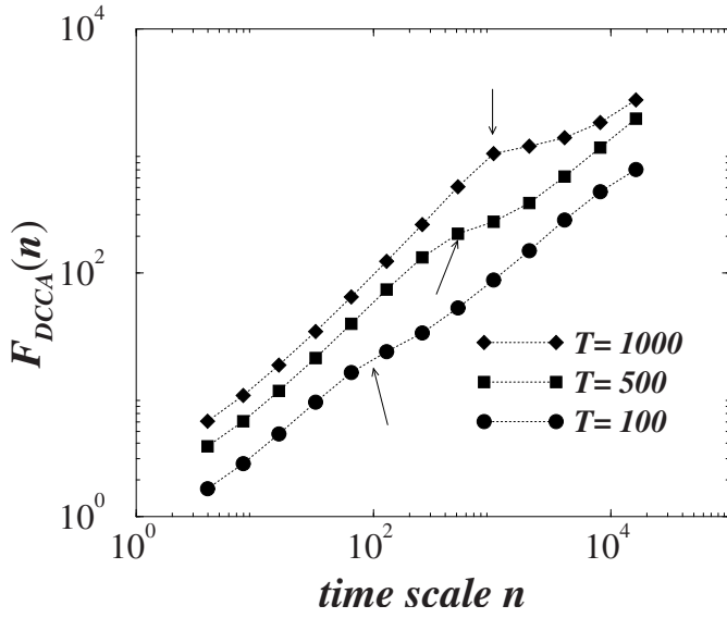
Fig. 6. Crossovers in the detrended cross-correlation analysis function F_{DCCA}(n) , calculated for cross-correlated noise with a sinusoidal trend. The cross-correlated time series \{y_i\} and \{y'_i\} are generated by the periodic two-component ARFIMA process defined by equations (2a, 2b). For \rho = 0.4 , W = 0.5 , A_1 = A_2 = 0.3 , and varying period T , we find a crossover in the F_{DCCA}(n) function that increases with T approximately as n_{2CC} \propto T .
