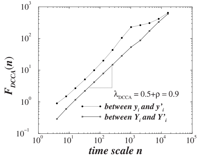
Fig. 7. DCCA function F_{DCCA}(n) after global and local sinusoidal detrending approaches. We generate two time series \{y_i\} and \{y'_i\} of the periodic two-component ARFIMA process of equations (2a, 2b) with \rho = \rho_1 = \rho_2 = 0.4 , W = 0.5 , A_1 = A_2 = 0.3 , and T_1 = T_2 = T = 10^3 . We see that F_{DCCA}(n) of y_i and y'_i exhibit a bump similar to that characteristic for DFA functions obtained for time series with periodic trends. After performing a global minimization of \sum_{i=1}^N (y_i - A_1 \sin(2\pi/Ti + \phi_1))^2 and \sum_{i=1}^N (y'_i - A_2 \sin(2\pi/Ti + \phi_2))^2 , we find the parameters of the first harmonic ( A_i, \phi_i, T_i ) in both time series \{y_i\} and \{y'_i\} . Then, we define two new time series, Y_i = y_i - A_1 \sin(2\pi/Ti + \phi_1) and Y'_i = y'_i - A_2 \sin(2\pi/Ti + \phi_2) . \{Y_i\} and \{Y'_i\} exhibit a “pure” power-law cross-correlation, with expected power-law exponent \lambda_{DCCA} = \lambda_{DFA} = 0.5 + \rho = 0.9 , since both time series are defined by the same \rho parameter.
