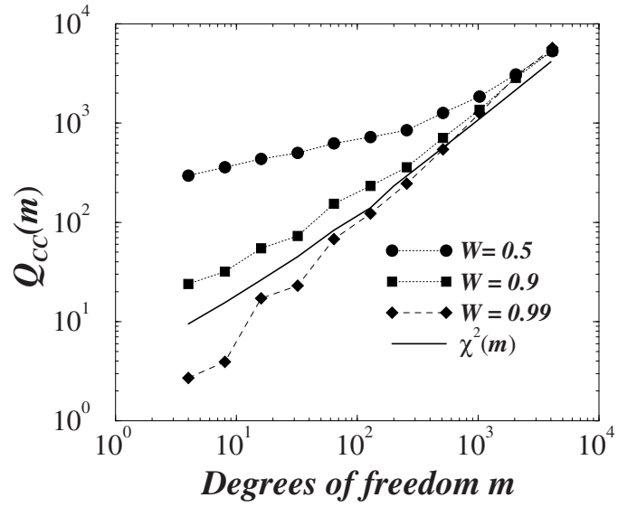
Fig. 5. Q_{CC}(m) versus the number of degrees of freedom m for different values of the cross-correlation coupling W . For each W , we generate one pair of time series \{y_i\} and \{y'_i\} defined by equations (2a, 2b). Each time series is comprised of N = 10^4 data points. There is no sinusoidal trend, so A_1 = A_2 = 0 . We also show the curve of the critical values of \chi^2(m) distribution at the 5% level of significance. Parameters are \rho_1 = 0.2 and \rho_2 = 0.4 . For W = 0.5 , the cross-correlations between \{y_i\} and \{y'_i\} are strongest and, for a wide range of m values, the curve of the test statistic of equation (6) for W = 0.5 is above all other curves including the curve of the critical values of \chi^2(m) distribution. For values of W very close to 1, the cross-correlations between \{y_i\} and \{y'_i\} become very weak, below the curve of the critical values of \chi^2(m) distribution.
