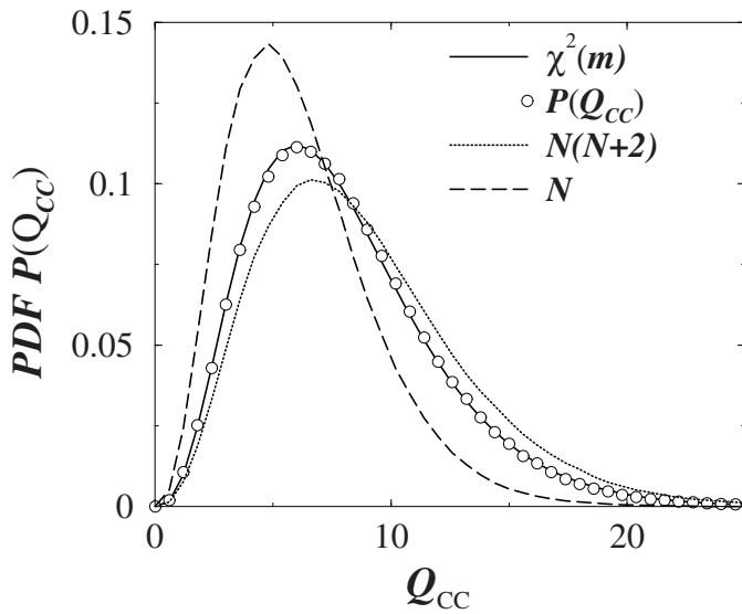
Fig. 1. Probability distribution function (pdf) P(Q_{CC}) of Q_{CC} defined in equation (6) together with the \chi^2(m) pdf, where m are the degrees of freedom. We also show P(Q') of Q' defined in equation (7). We generate 10^6 pairs of time series \{y_i\} and \{y'_i\} , where each time series is generated by an i.i.d. Gaussian process with mean zero and unit variance. Each time series is comprised of N = 20 data points (small time series). We choose m = 8 , and for each pair of time series we calculate the cross-correlations X_i , where i = 1, \dots, 8 . We find a perfect match between P(Q_{CC}(m)) and \chi^2(m) . In opposite, the pdf of Q' defined in equation (7) deviates from the \chi^2(m) distribution. We also show the pdf of a test defined as N \sum_i^m X_i^2 , which substantially deviates from \chi^2(m) .
