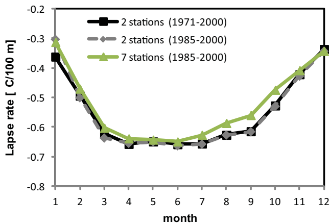
Fig. 3. Comparison of surface temperature lapse rate calculations derived from two and seven stations.
