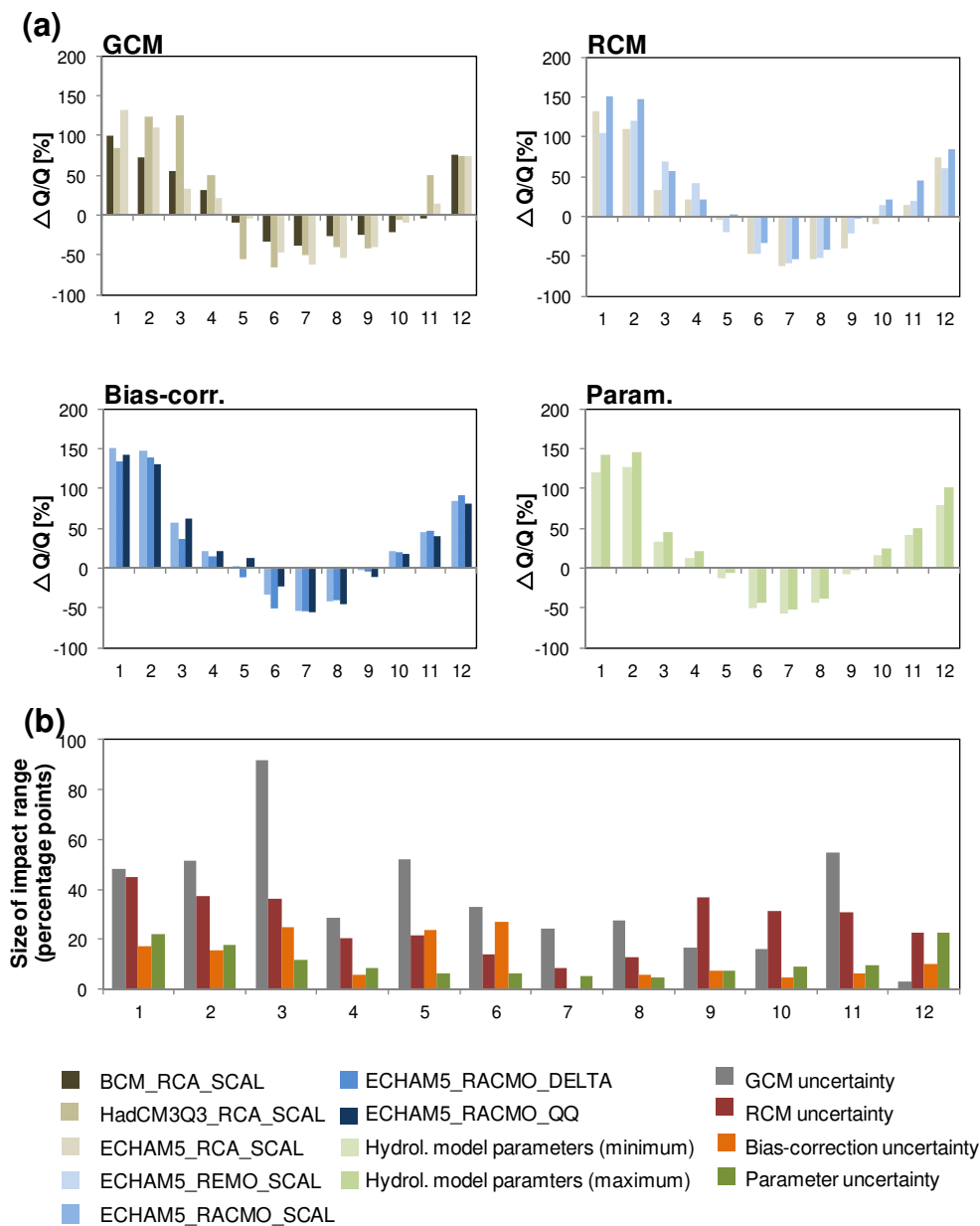
Fig. 8. (a) Uncertainty in the projections of mean monthly runoff ( Q ) resulting from GCM, RCM, bias-correction and hydrological model parameters. (b) Size of impact range originating from each uncertainty source. The differences (percentage points) between the minimum and maximum values are plotted.
