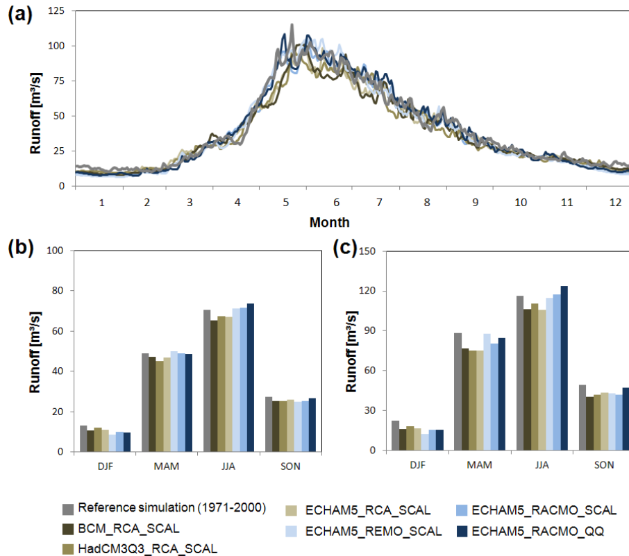
Fig. 5. Runoff from HQsim simulations using observed station data (reference simulation) and the different modelling chains showing (a) mean daily runoff, (b) mean seasonal runoff and (c) the mean seasonal 90 %-quantile of daily runoff.
