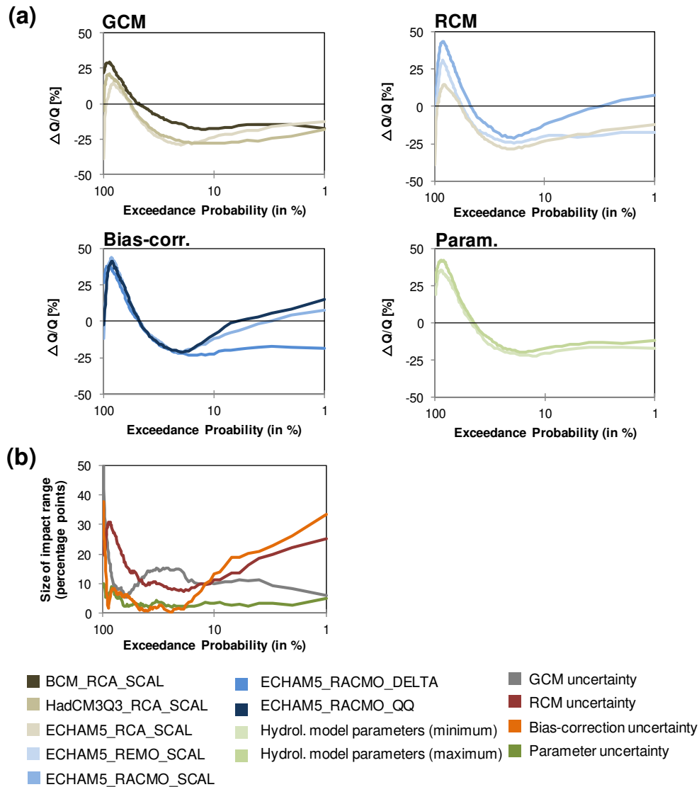
Fig. 9. (a) Uncertainty in flow exceedance probabilities resulting from GCM, RCM, bias-correction and hydrological model parameters. (b) Size of impact range originating from each uncertainty source. The differences (percentage points) between the minimum and maximum values are plotted.
