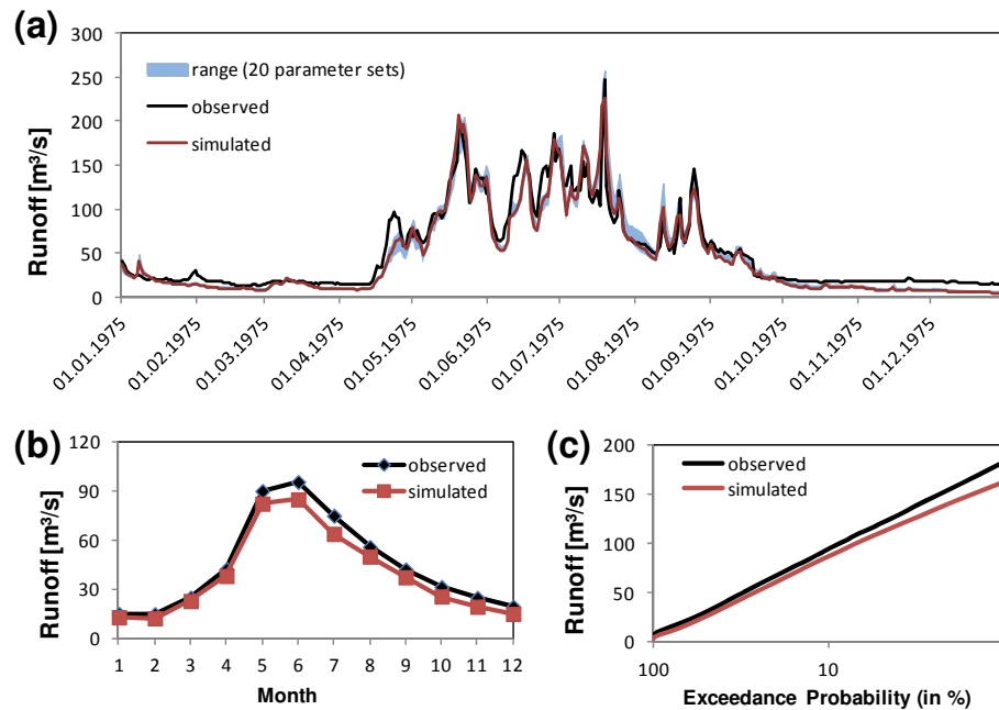
Fig. 4. (a) Observed and HQsim simulated runoff for the year 1975. The blue shading indicates the range obtained when using 20 different parameter sets. (b) Mean monthly runoff and (c) exceedance probability distribution for observed and simulated data, based on the period from 1971 to 2005.
