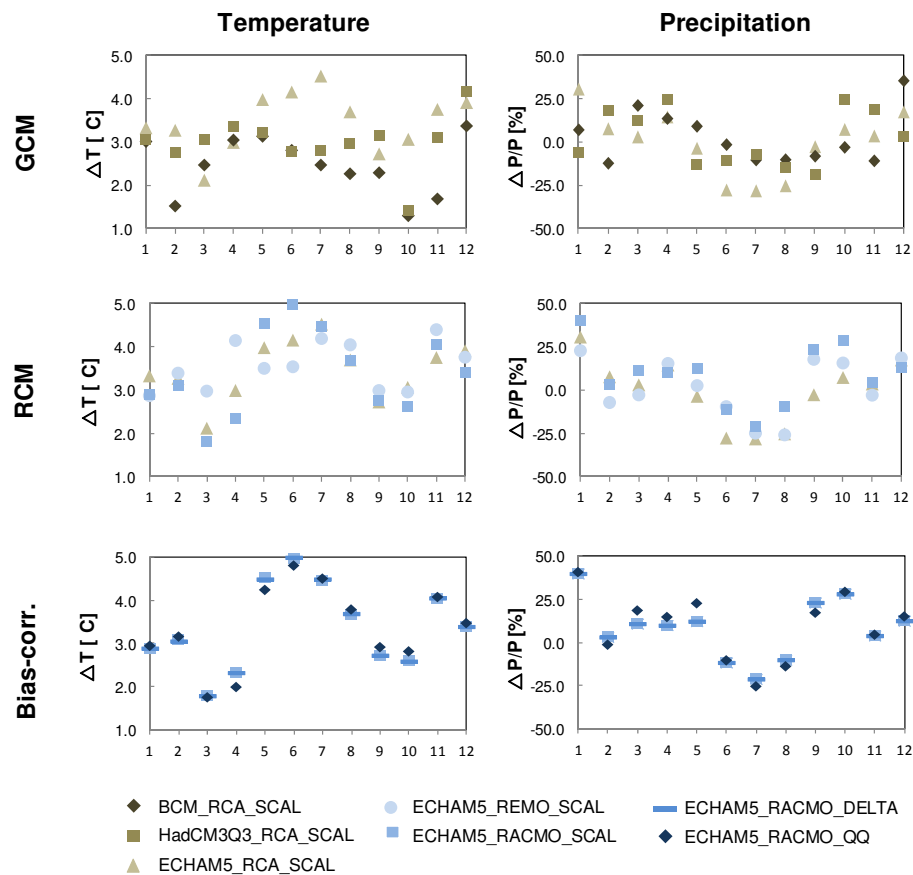
Fig. 6. Mean monthly changes in temperature ( T ) and precipitation ( P ) between the reference period (1971–2000) and the future scenario (2070–2099). Uncertainty originating from GCM, RCM and bias-correction is illustrated. Temperature and precipitation data are averaged across the catchment.
