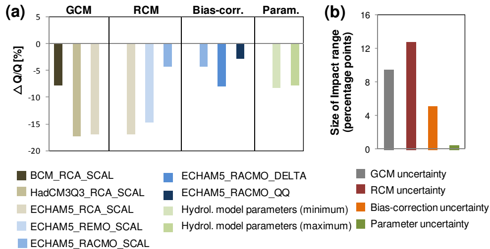
Fig. 7. (a) Uncertainty in the projection of mean annual runoff ( Q ) resulting from GCM, RCM, bias-correction and hydrological model parameters. (b) Size of impact range originating from each uncertainty source. The differences (percentage points) between the minimum and maximum values are plotted.
