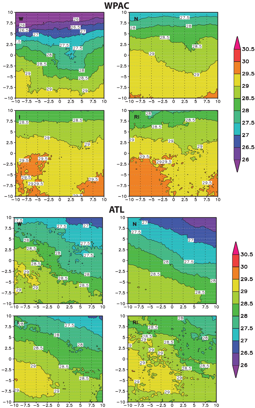
FIG. 8. As in Fig. 5, but for TMI sea surface temperature: T_{sea} ( ^{\circ} C).
