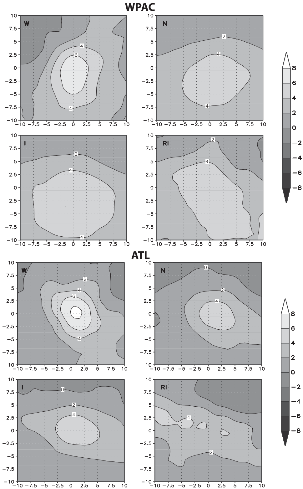
FIG. 13. As in Fig. 5, but for NOGAPS 200-hPa divergence: \nabla \cdot \mathbf{u}_{200}^f ( 10^{-6} \text{ s}^{-1} ).
