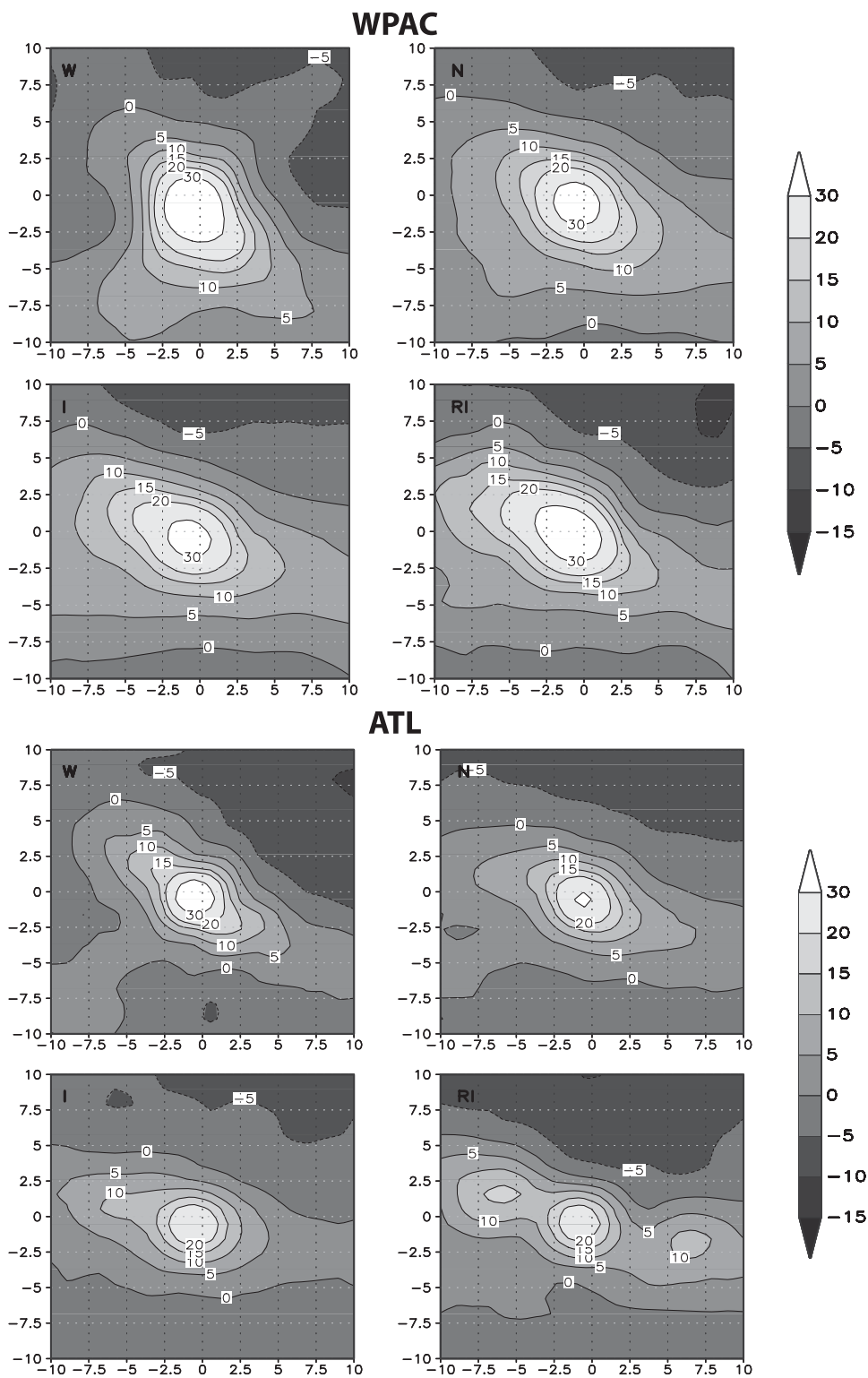
FIG. 14. As in Fig. 5, but for NOGAPS 850-hPa filtered relative vorticity: \mathbf{k} \cdot \mathbf{V} \times \mathbf{u}_{850}^f ( 10^{-6} \text{ s}^{-1} ).
