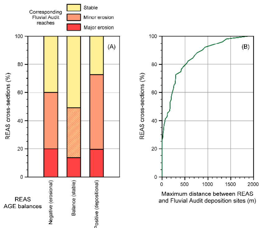
Figure 3. (A) Comparison between REAS (River Energy Audit Scheme) Annual Geomorphic Energy (AGE) balances and corresponding Fluvial Audit reaches in the River Kent drainage basin, UK (refer also to Figure 1). As there are no Fluvial Audit reaches classified as entirely depositional, positive AGE balances lie within either stable or erosional reaches [188]. The Fluvial Audit reaches classified as minor erosion that correspond to stable REAS locations (hatched) conceivably refer to sites with generally stable bed and banks but with a degree of erosion along the banklines associated with washout between trees and cattle poaching and are thus unlikely to be indicative of system-wide instability; (B) Proximity of REAS sites with positive balances (depositional) to areas of deposition mapped in the Fluvial Audit.
