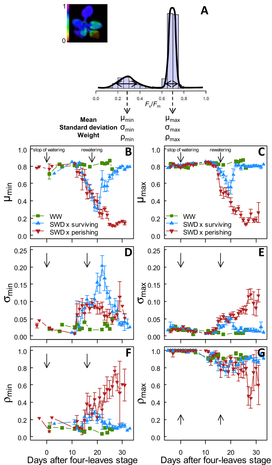
Figure 3 Dynamics of the parameters describing the bimodal distributions. (A) Example of a bimodal distribution composed of two clusters of pixels grouping in two modes. The higher mode (max; with the highest F_v/F_m values) represents the healthiest parts of the rosette whereas the second mode (min; with the lowest F_v/F_m values) represents damaged/senescing parts of the rosette. Each mode i of the mixture distribution of F_v/F_m values is characterized by mean \mu_i , standard deviation \sigma_i and weight \rho_i . (B-G) Dynamics of \mu_{\max} and \mu_{\min} of F_v/F_m values, \sigma_{\max} and \sigma_{\min} , and \rho_{\max} and \rho_{\min} in well-watered (WW) plants and under severe water stress (SWD; surviving and perishing plants) as a function of days after four-leaves stage (beginning of SWD) until bolting. Data are means ( \pm SE) of 13–29 plants.
