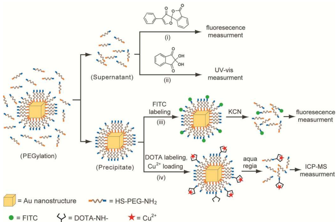
Figure 1. Schematic illustration of the four methods for quantifying the average number of -S-PEG-NH 2 chains on the surface of one single Au nanostructure: i ) fluorescamine-based assay, ii ) ninhydrin-based assay, iii ) FITC-labeling assay, and iv ) Cu 2+ -labeling assay.
