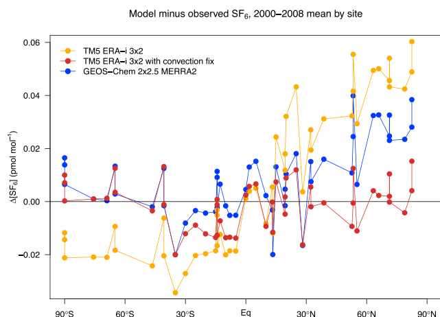
Figure 5. The 9-year average model-minus-observed residuals of SF 6 at the marine boundary layer sites listed in Table S1, arranged by latitude. Results are from two different versions of TM5 with ERA-i meteorology (gold, an earlier version subject to a fault in convective transport; red, a version correcting that fault) and GEOS-Chem using MERRA2 (blue).
