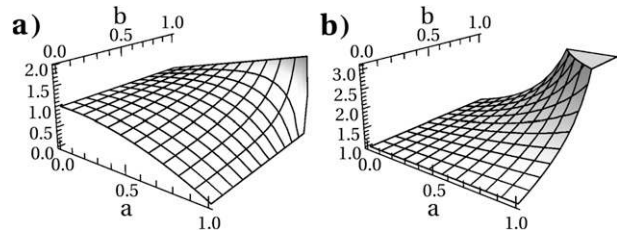
FIG. 4. (a) Plots of quotients B_X/B'_X = (1 - a^2)/(1 - ab) for a contemporaneous regression [case (i)] and (b) B_{X_{t-1}}/B'_{X_{t-1}} = 1/(1 - ab) for a lagged regression [case (ii)]. These quotients describe the factor by which the regression coefficients are altered due to autocorrelations a and b . Note that the quotient B_{X_{t-1}}/B'_{X_{t-1}} goes to infinity for a = b = 1 . The plots demonstrate the strong nonlinear dependence of univariate regressions on autocorrelation.
