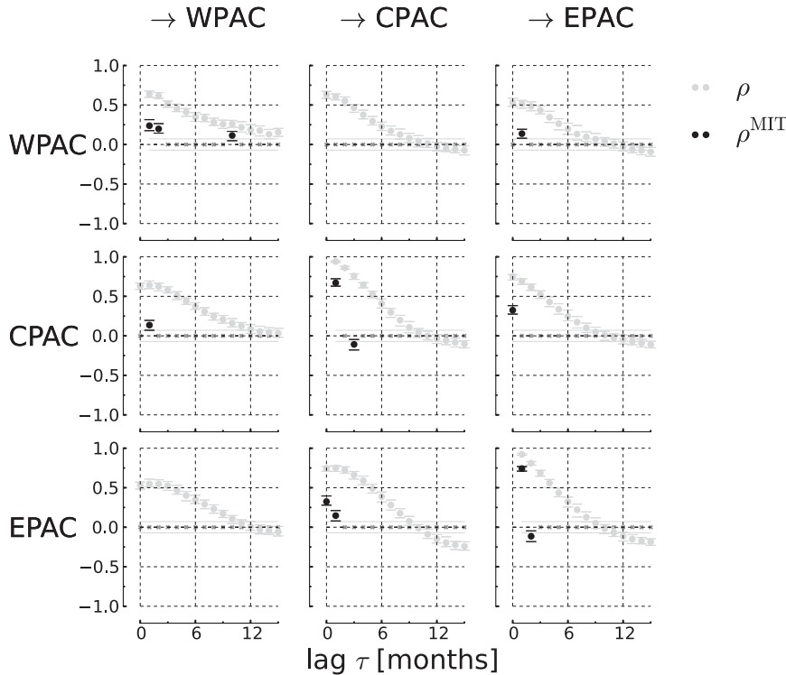
FIG. 9. Cross correlation (gray) and significant MIT values (black) for all pairs of variables (WPAC, CPAC, and EPAC). For example, here MIT for the link CPAC → WPAC is the partial correlation \rho(C_{t-1}; W_t | \mathcal{P}_{W_t} \setminus \{C_{t-1}\}, \mathcal{P}_{C_{t-1}}) with parents as given in the main text. The most important finding is the vanishing link EPAC → WPAC, which shows that the influence of the east on the west Pacific is mediated via the surface of the equatorial central Pacific. On the other hand the link WPAC → EPAC stays, implying that this influence was not mediated via this region.
