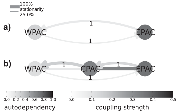
FIG. C1. Ensemble statistics of sliding window analysis of the bi- and trivariate Walker circulation examples. This kind of graph has been termed process graph in Runge et al. (2012b) that aggregates the information in the time series graph. The node shade denotes the ensemble average auto-MIT lag-1 strength and the link shade encodes the ensemble average MIT strength at the lag denoted in the link label. The link width, on the other hand, is proportional to the fraction of sliding windows with this link being significant.
