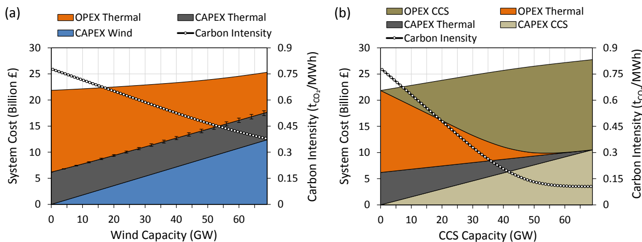
Fig. 10 Total system cost as sum of capital (CAPEX) and operational expense (OPEX) and the overall Carbon Intensity (CI) for (a) thermal-wind and (b) thermal-CCS integrated system. In (a), OPEX decreases with reduced fuel consumption and utilisation; CAPEX increase with wind power installation. The error bars indicate the sensitivity in thermal CAPEX referring to the low and high CC values from figure 8. The CI reaches 0.4 t_{CO_2}/MWh at the maximum wind power deployment. In (b), thermal CAPEX and OPEX decrease according to the increase of the respective CCS cost components. The system CI reduces to 0.1 t_{CO_2}/MWh at the maximum share of CCS-equipped capacity.
