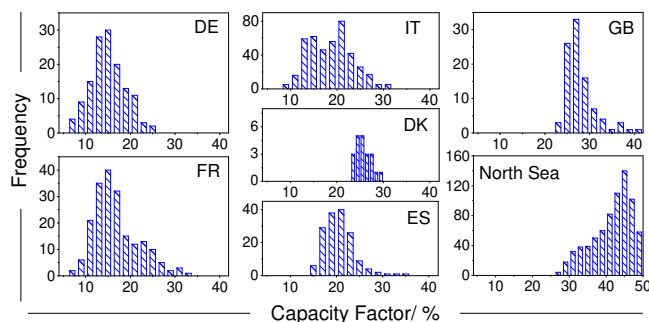
Fig. 6 Histogram of long-run capacity factors averaged over 1995-2014 and aggregated for selected European countries from data for single turbines by location 116,117 . The visualised data for the selected countries does not include offshore areas. The North Sea refers only to British territorial waters, and is presented on a different x-axis scale.
