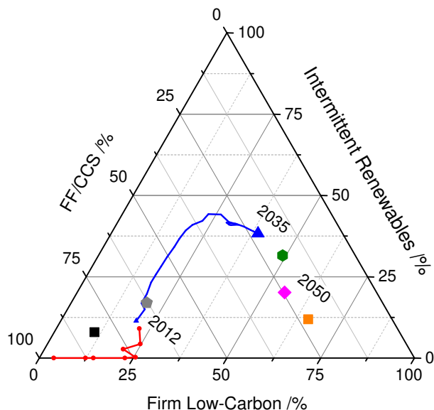
Fig. 4 Equivalent data as figure 3; Transition of electricity generation by fuel for 1960 to 2012 according to the IEA, and 2012 to 2035 to DECC's reference scenario 73 . Remaining scenarios are shown with large markers for the respective 2050 fuel mix.
