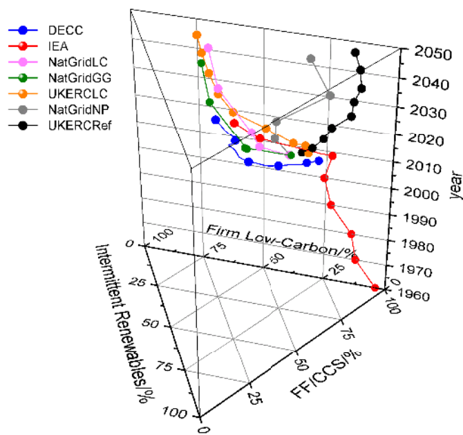
Fig. 3 Trajectories for electricity generation by fuel in a technology ternary, data from 70,72,73,115 . FF/CCS refers to fossil-fuelled generators with and without CCS, and firm low-carbon includes imports, which come predominantly from nuclear-rich France and hydro-rich Norway. Data is normalised to total electricity generation for each year or according to the time discretisation of the given set.
