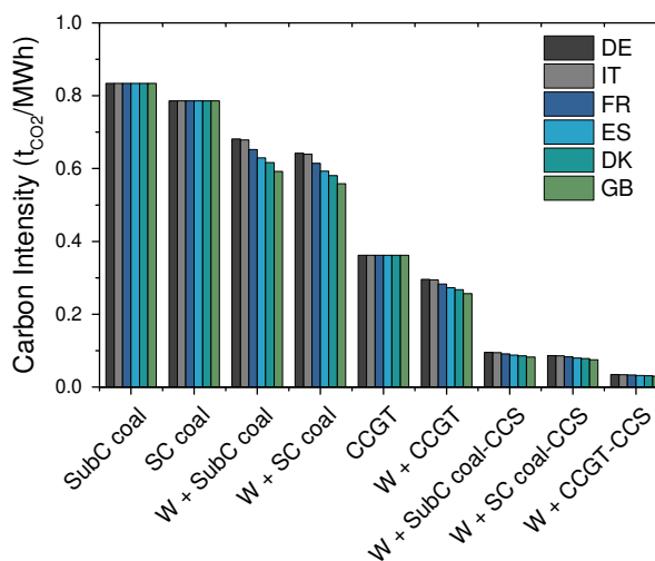
Fig. 7 Carbon Intensity for different system setups derived with the IECM tool 85 . “SubC coal” represents a subcritical coal power plant (gross electricity output 650 MW, net plant efficiency 37.84 %), “SC coal” a supercritical coal power plants (gross electricity output 650 MW, net plant efficiency 40.16 %), and CCGT a natural gas combined cycle power plant (gross electricity output 298 MW, net plant efficiency 50.33 %). All CCS systems are set to capture 90 % of flue gas CO 2 . The energy penalty of post-combustion CCS (using a 30 wt% monoethanolamine solvent) reduces plant efficiencies to 27.11 % (SubC), 29.84 % (SC) and 43.41 % (CCGT). The CF for on-shore wind (W) is set to the annual average for each country 84 .
