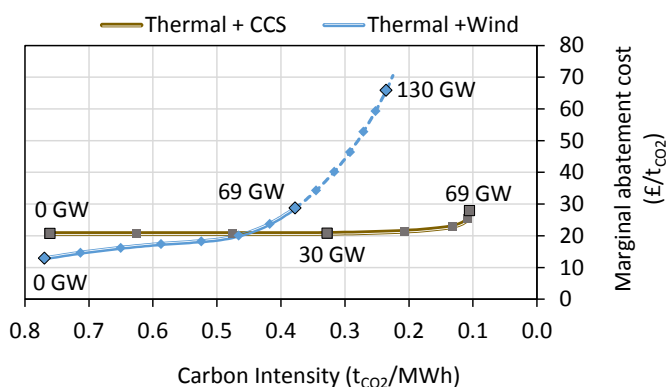
Fig. 11 Reduction in Carbon Intensity (CI) in the hypothetical thermal-CCS and thermal-wind systems. The continuous lines with markers refer to the systems in figures 9 and 10, where CCS and wind respectively are deployed up to a level of 69 GW. The dashed line for the wind capacity integrated systems represents the theoretical continuation of increasing wind capacity and thermal back-up in order to achieve a CI of 0.225 t_{CO_2}/MWh .
