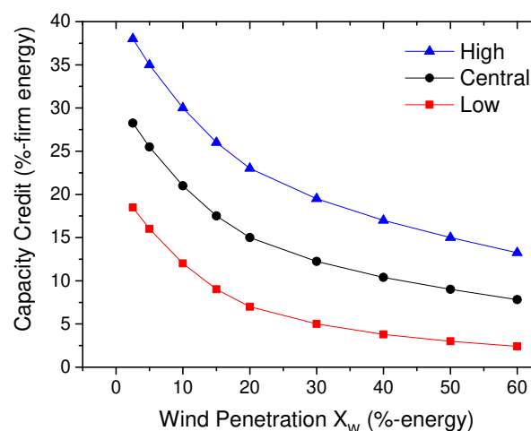
Fig. 8 Capacity credit of wind power generators, based on data presented by Gross et al. 75 and references therein. It can be observed that initial deployment of wind power can contribute between 17 - 37 % of its firm capacity, but that this capacity credit reduces with increasing deployment.
