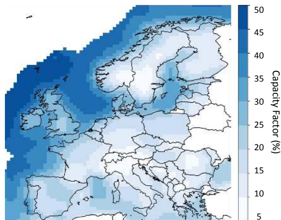
Fig. 5 Long-run capacity factors (CFs) averaged over 1995-2014 and aggregated across Europe 116,117 . The CFs determined from hourly wind speeds using the Renewables.Ninja database 84 , assuming 80 metre tall Vestas V80 2MW turbines were installed at regularly-spaced locations on land and up to 250 km out to sea.
