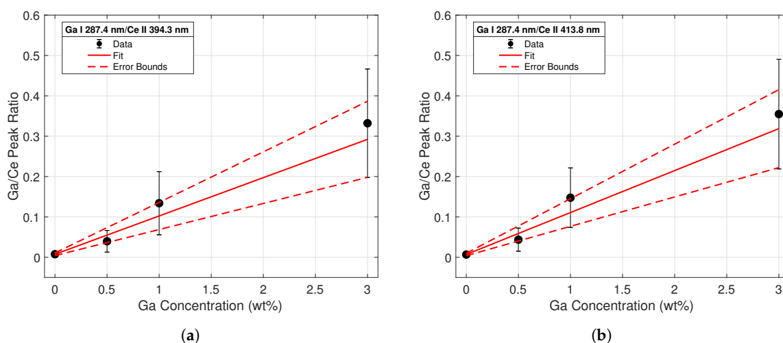
Figure 5. Calibration curve from line intensity ratios of the Ga I 287.4-nm emission to the (a) Ce II 394.3 nm (b) and the Ce II 413.8-nm emission lines. The regression fit is shown with a solid red line, while errors in the regression coefficients are plotted with the dashed red lines.
