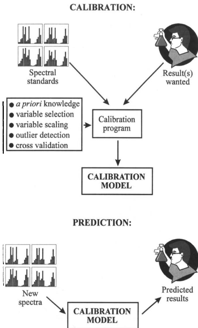
Fig. 1. The process of multivariate calibration via supervised learning consists of two stages. Calibration: establishing a CALIBRATION MODEL for later prediction of “results” (e.g., amount of determinand) from “spectra” by matching spectral standards and the known results wanted from a set of calibration samples (the training set) in some sort of supervised learning calibration program; this may be by using a neural network simulation, or with a program that performs multiple linear regression, partial least squares or principal component regression. Some background knowledge may be used in the formation of the model such as a priori knowledge, variable selection and scaling, outlier detection and cross validation.
