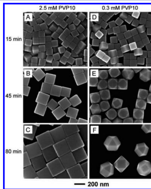
Figure 6. SEM images of Ag polyhedrons grown from 100 nm cubic seeds in the presence of (A–C) 2.5 mM and (D–F) 0.3 mM PVP10 as the capping agent. The samples were collected from the reaction solutions at different reaction times: (A, D) 15 min, (B, E) 45 min, and (C, F) 80 min, respectively.
