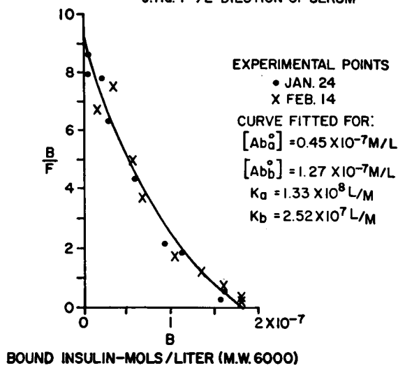
FIG. 11. \frac{B}{F} vs. B IN SERUM OF SUBJECT J. HA.
