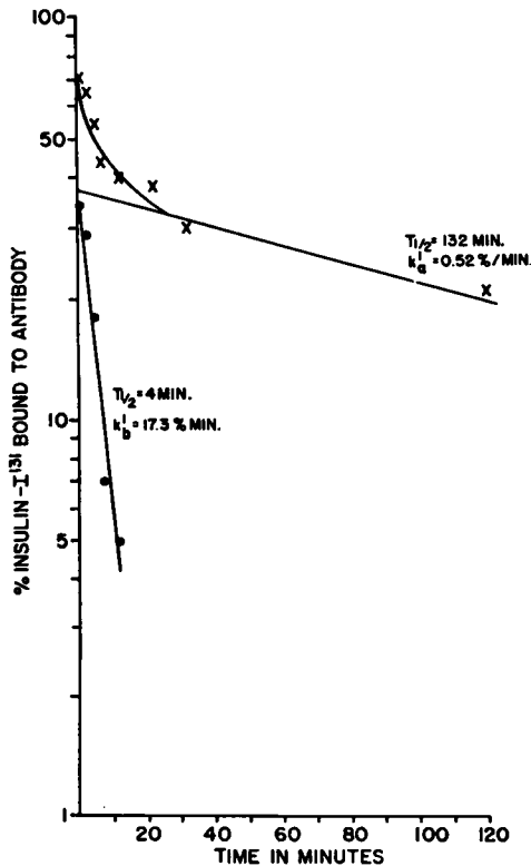
RATE OF DISSOCIATION OF Ag-Ab COMPLEX DETERMINED FROM CHROMATOGRAPHIC SEPARATION OF BOUND & UNBOUND INSULIN
