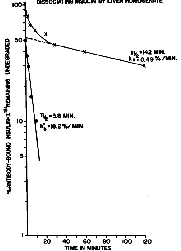
FIG. 9. RATE OF DISSOCIATION OF INSULIN-I 131 -ANTIBODY COMPLEXES IN SERUM OF SUBJECT RU.: a) DETERMINED BY PAPER CHROMATOGRAPHY; b) DETERMINED FROM RATE OF DEGRADATION BY LIVER INSULINASE
