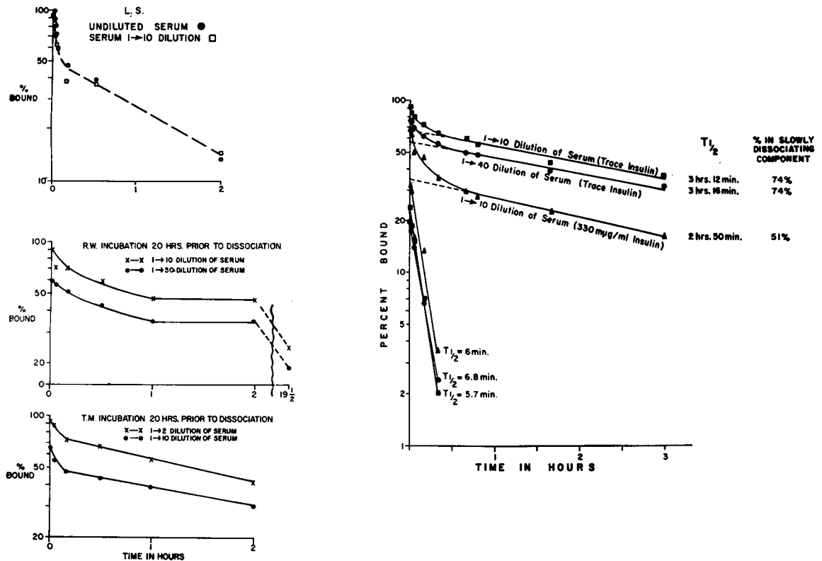
FIG. 12. "DISSOCIATION" OF INSULIN-ANTIBODY COMPLEXES FORMED AT DIFFERENT DILUTIONS OF THE SAME ANTISERUMS
