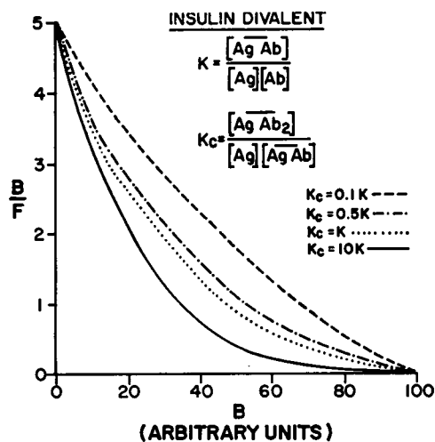
FIG. 3. SCHEMATIC PLOTS OF \frac{B}{F} vs. B FOR DIVALENT INSULIN REACTING WITH A SINGLE ORDER OF ANTIBODY COMBINING-SITES AT DIFFERENT \frac{K_c}{K} RATIOS
