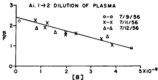
BOUND INSULIN-MOLS/LITER (M.W. 6000)
