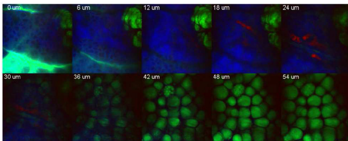
Figure 4. Multiplex SRS z stack images of freshly excised mouse ear skin tissue: red - blood contrast, green - lipid contrast, and blue - protein contrast. Each image is 512×512 pixels.
