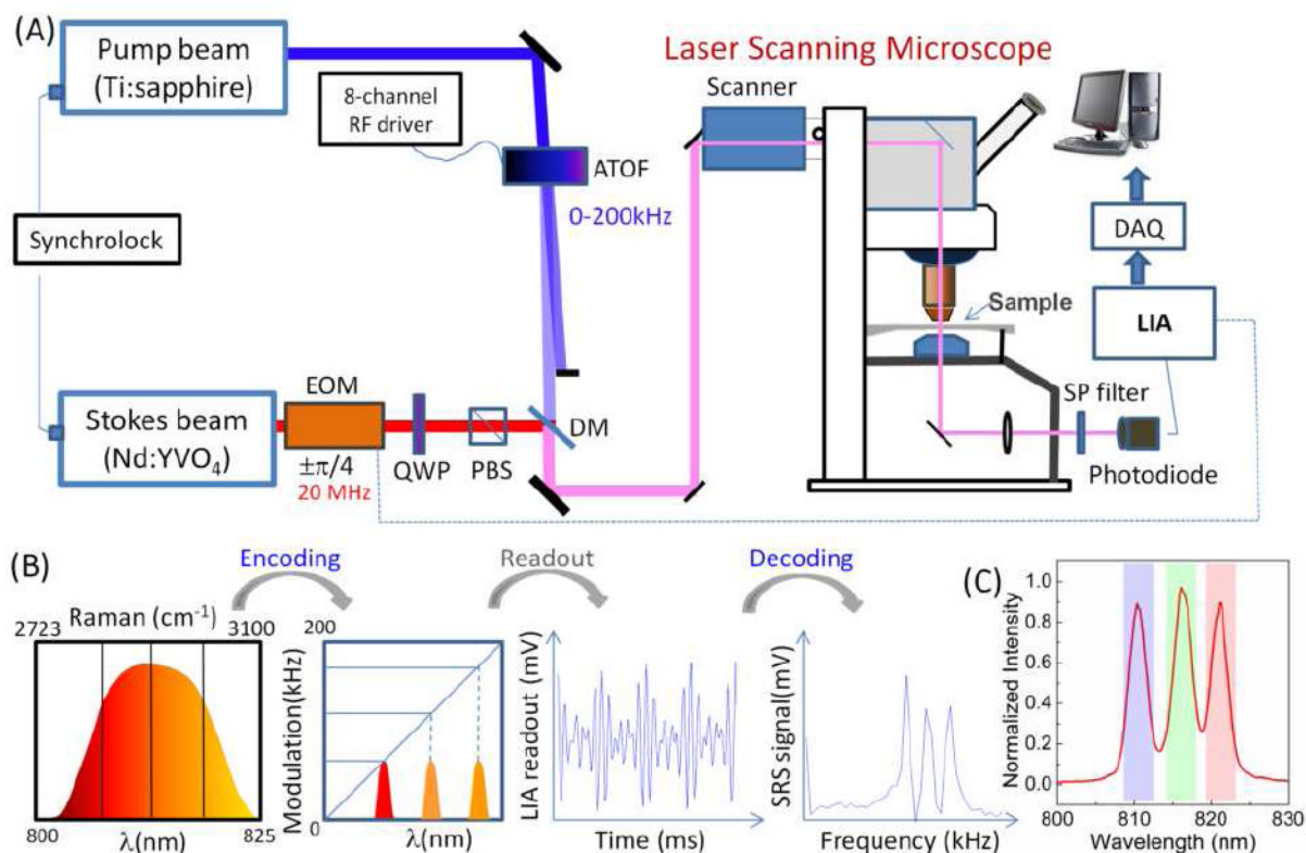
Figure 1. (A) Schematic diagram of multiplex SRS setup. HWP: half-wave plate; QWP: quarter-wave plate; EOM: electro-optical modulator; PBS: polarizing beamsplitter; DM: dichroic mirror; PMT: photomultiplier tube; LIA: lock-in amplifier. (B) Workflow of the multiplex Raman encoding and decoding process. (C) Example AOTF filtered spectrum using three channel modulation. Each shaded region corresponds to one channel modulated at a different frequency.
