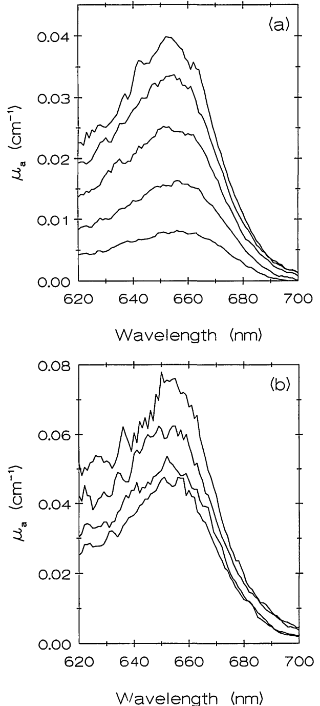
Fig. 5. Spectra of MB absorption coefficients at different MB concentrations in the Liposyn solution. The various spectra refer to MB concentrations of (a) 0.045, 0.090, 0.135, 0.180, and 0.225 \mu\text{M} ; (b) 0.270, 0.315, 0.360, and 0.450 \mu\text{M} . The spectrum relative to 0.405 \mu\text{M} is not shown for clarity.
